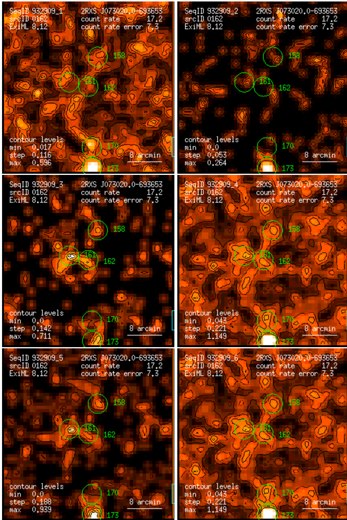
Figure 162: RASS 932909: detection 0162: band rate images, Gaussian filter: (1) PSPC channels 11 – 41, (2) 52 – 90, (3) 91 – 201, (4) 11 – 235, (5) 52 – 201, (6) 11 – 201. Broad band rates in counts/ks. Band rate contour levels in counts/ks/arcmin 2 .
