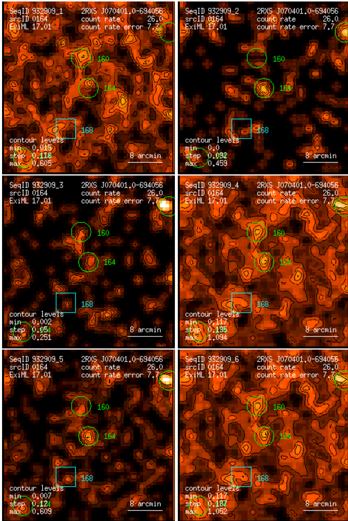
Figure 164: RASS 932909: detection 0164: band rate images, Gaussian filter: (1) PSPC channels 11 – 41, (2) 52 – 90, (3) 91 – 201, (4) 11 – 235, (5) 52 – 201, (6) 11 – 201. Broad band rates in counts/ks. Band rate contour levels in counts/ks/arcmin 2 .
