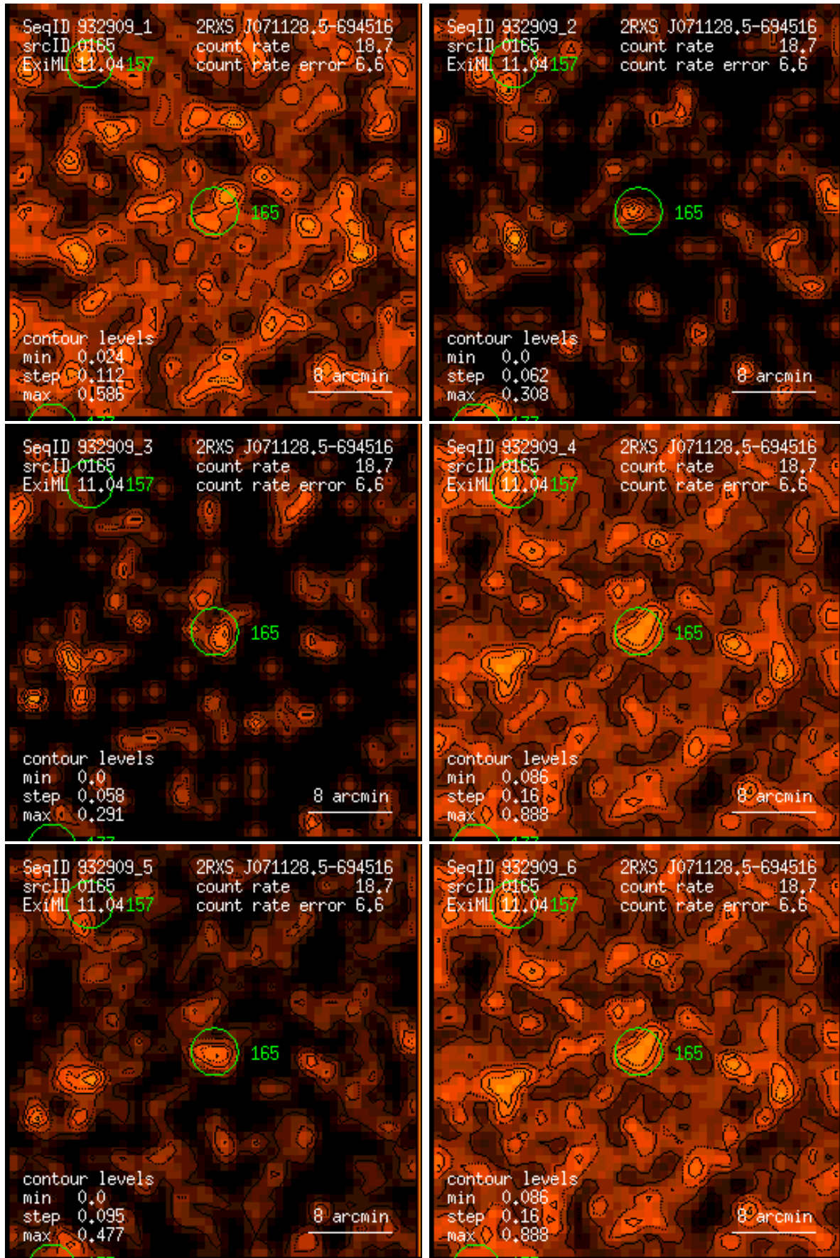
Figure 165: RASS 932909: detection 0165: band rate images, Gaussian filter: (1) PSPC channels 11 – 41, (2) 52 – 90, (3) 91 – 201, (4) 11 – 235, (5) 52 – 201, (6) 11 – 201. Broad band rates in counts/ks. Band rate contour levels in counts/ks/arcmin 2 .
