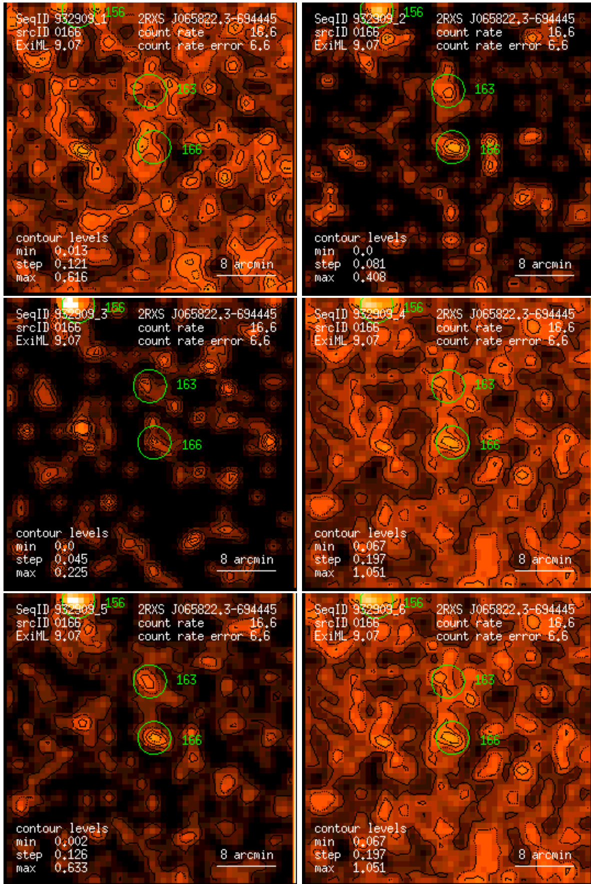
Figure 166: RASS 932909: detection 0166: band rate images, Gaussian filter: (1) PSPC channels 11 – 41, (2) 52 – 90, (3) 91 – 201, (4) 11 – 235, (5) 52 – 201, (6) 11 – 201. Broad band rates in counts/ks. Band rate contour levels in counts/ks/arcmin 2 .
