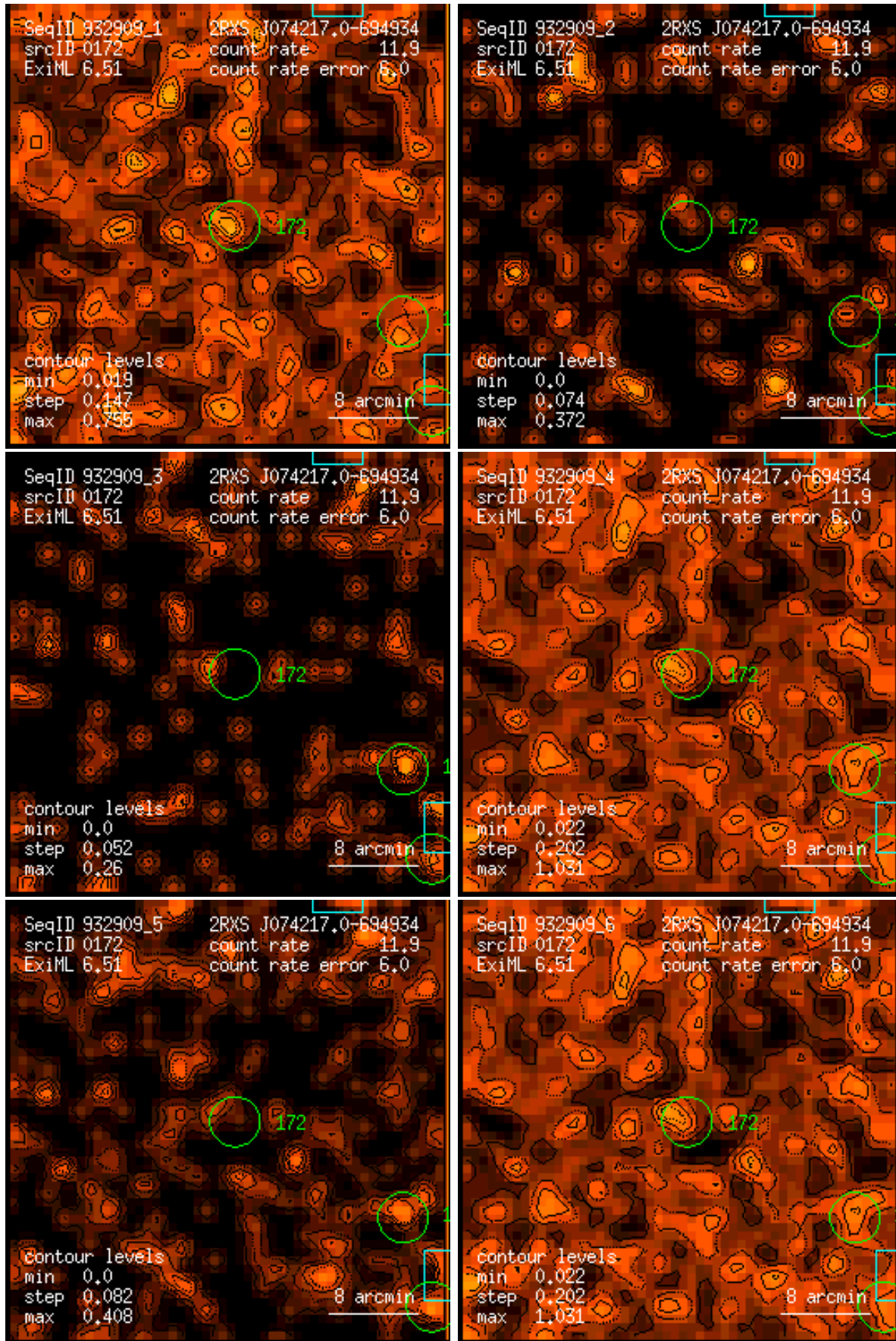
Figure 172: RASS 932909: detection 0172: band rate images, Gaussian filter: (1) PSPC channels 11 – 41, (2) 52 – 90, (3) 91 – 201, (4) 11 – 235, (5) 52 – 201, (6) 11 – 201. Broad band rates in counts/ks. Band rate contour levels in counts/ks/arcmin 2 .
