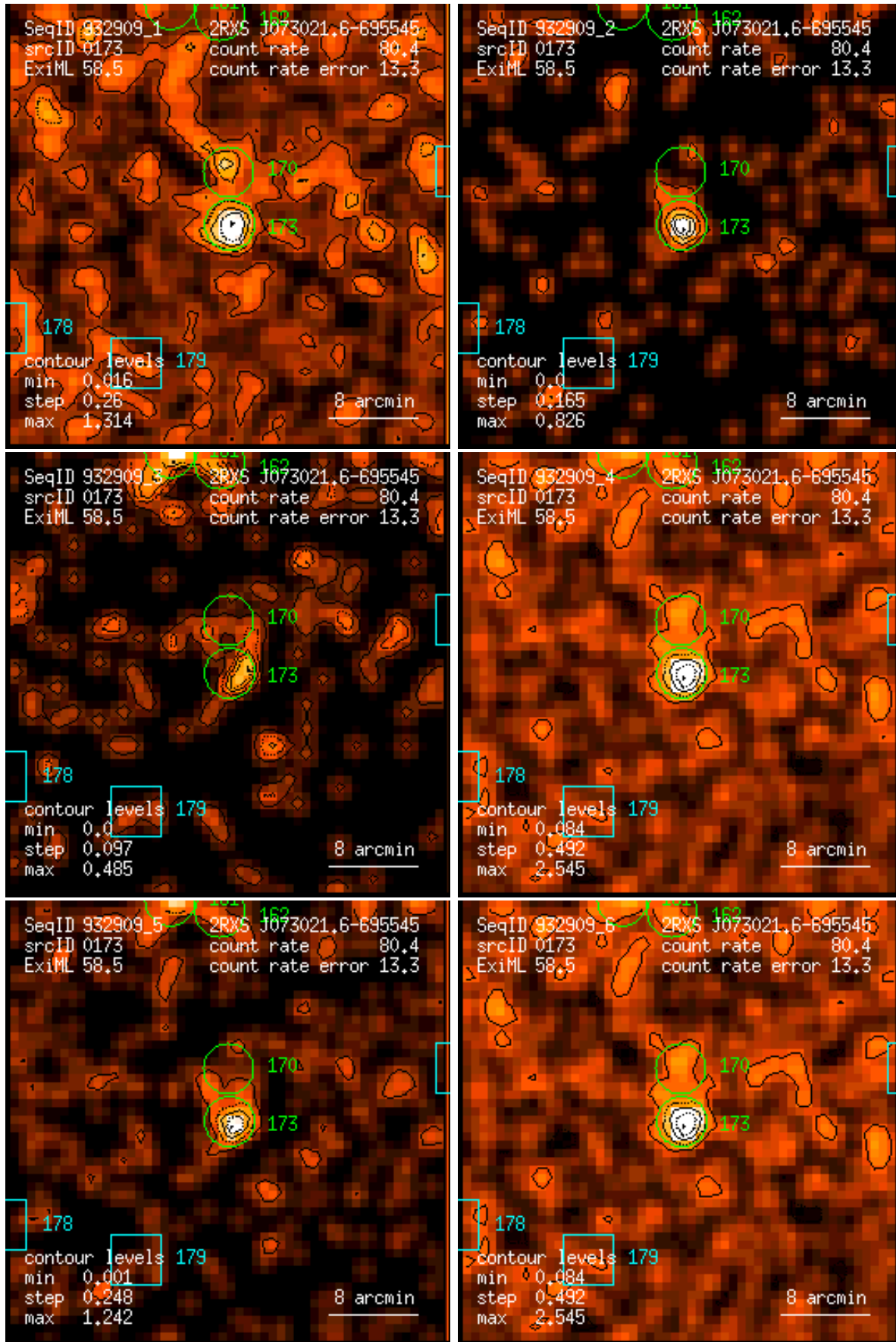
Figure 173: RASS 932909: detection 0173: band rate images, Gaussian filter: (1) PSPC channels 11 – 41, (2) 52 – 90, (3) 91 – 201, (4) 11 – 235, (5) 52 – 201, (6) 11 – 201. Broad band rates in counts/ks. Band rate contour levels in counts/ks/arcmin 2 .
