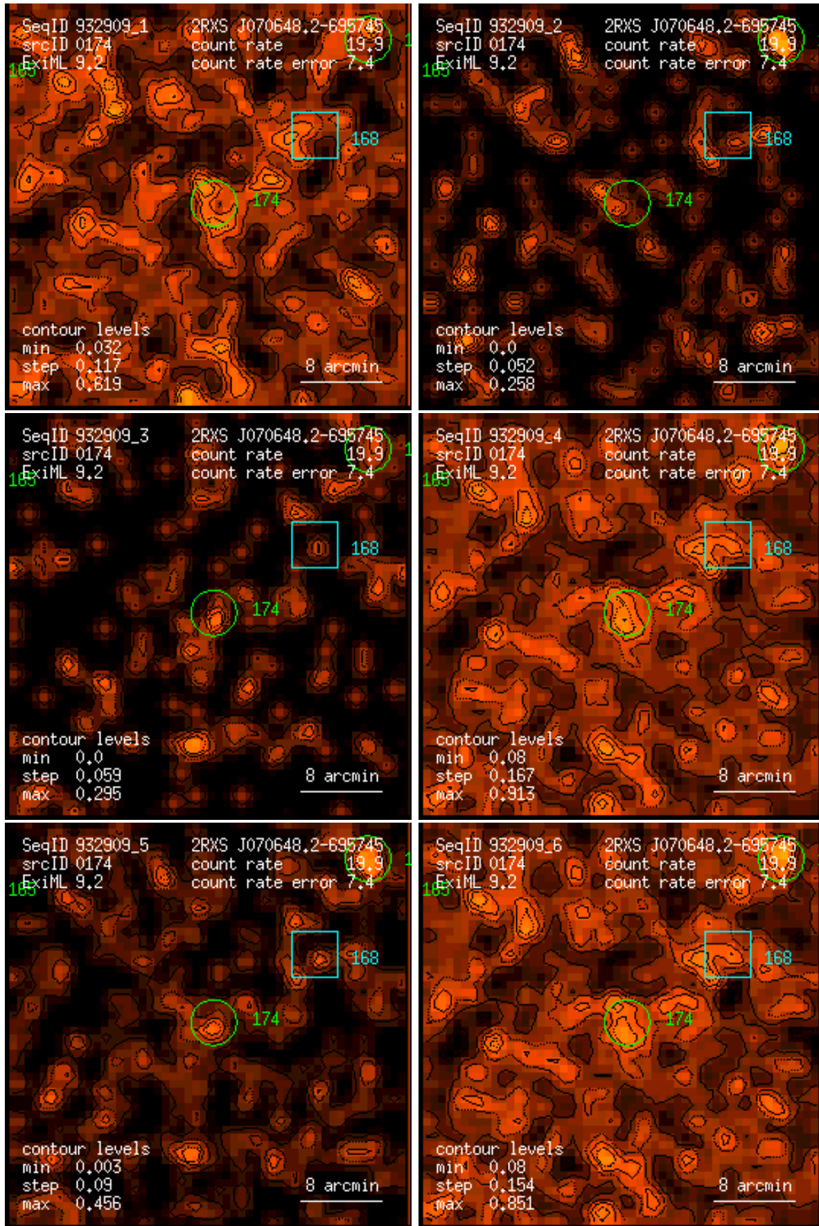
Figure 174: RASS 932909: detection 0174: band rate images, Gaussian filter: (1) PSPC channels 11 – 41, (2) 52 – 90, (3) 91 – 201, (4) 11 – 235, (5) 52 – 201, (6) 11 – 201. Broad band rates in counts/ks. Band rate contour levels in counts/ks/arcmin 2 .
