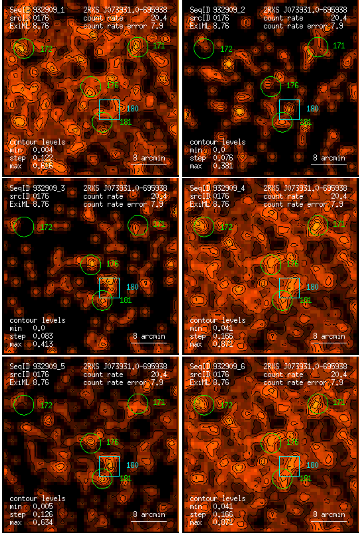
Figure 176: RASS 932909: detection 0176: band rate images, Gaussian filter: (1) PSPC channels 11 – 41, (2) 52 – 90, (3) 91 – 201, (4) 11 – 235, (5) 52 – 201, (6) 11 – 201. Broad band rates in counts/ks. Band rate contour levels in counts/ks/arcmin 2 .
