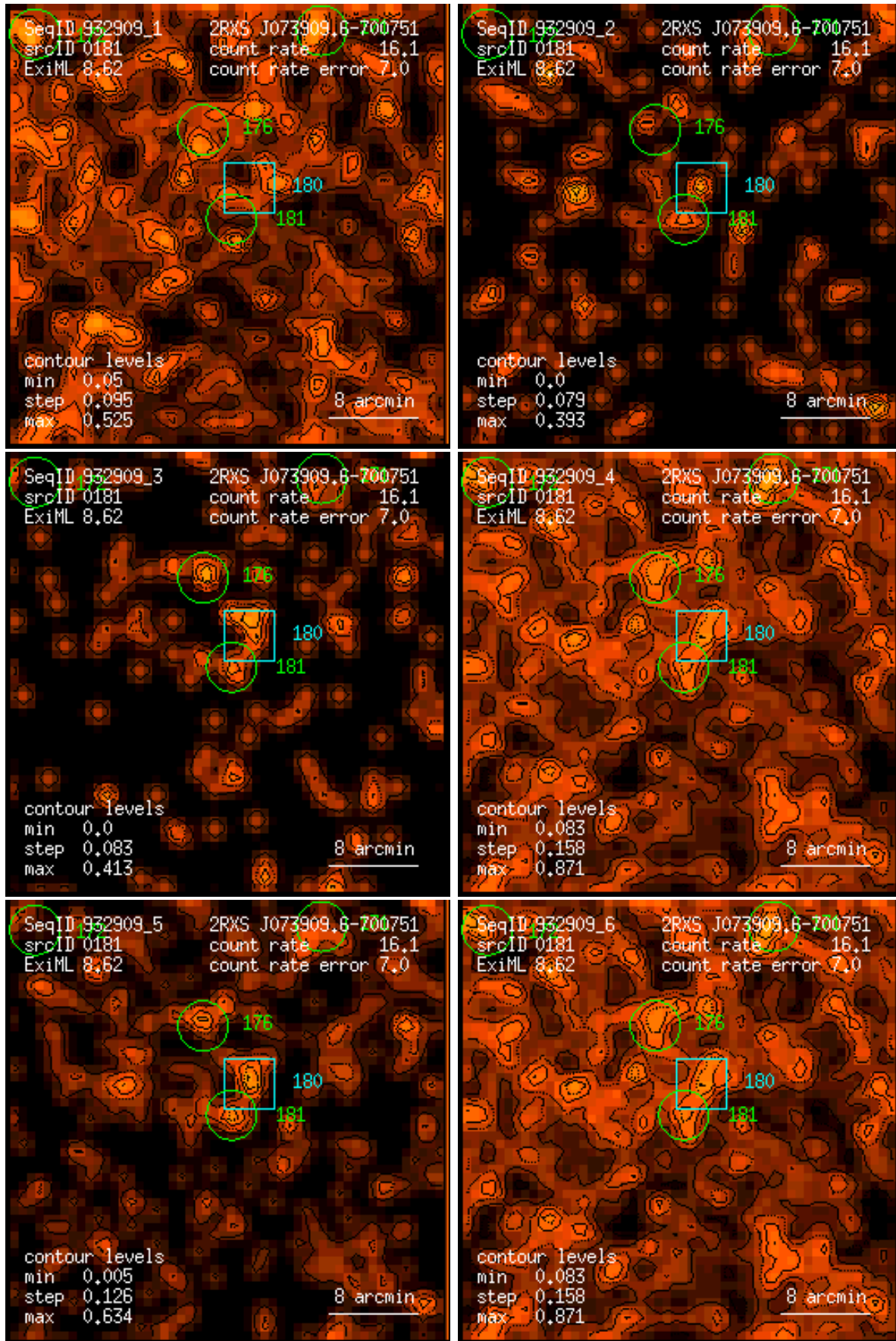
Figure 181: RASS 932909: detection 0181: band rate images, Gaussian filter: (1) PSPC channels 11 – 41, (2) 52 – 90, (3) 91 – 201, (4) 11 – 235, (5) 52 – 201, (6) 11 – 201. Broad band rates in counts/ks. Band rate contour levels in counts/ks/arcmin 2 .
