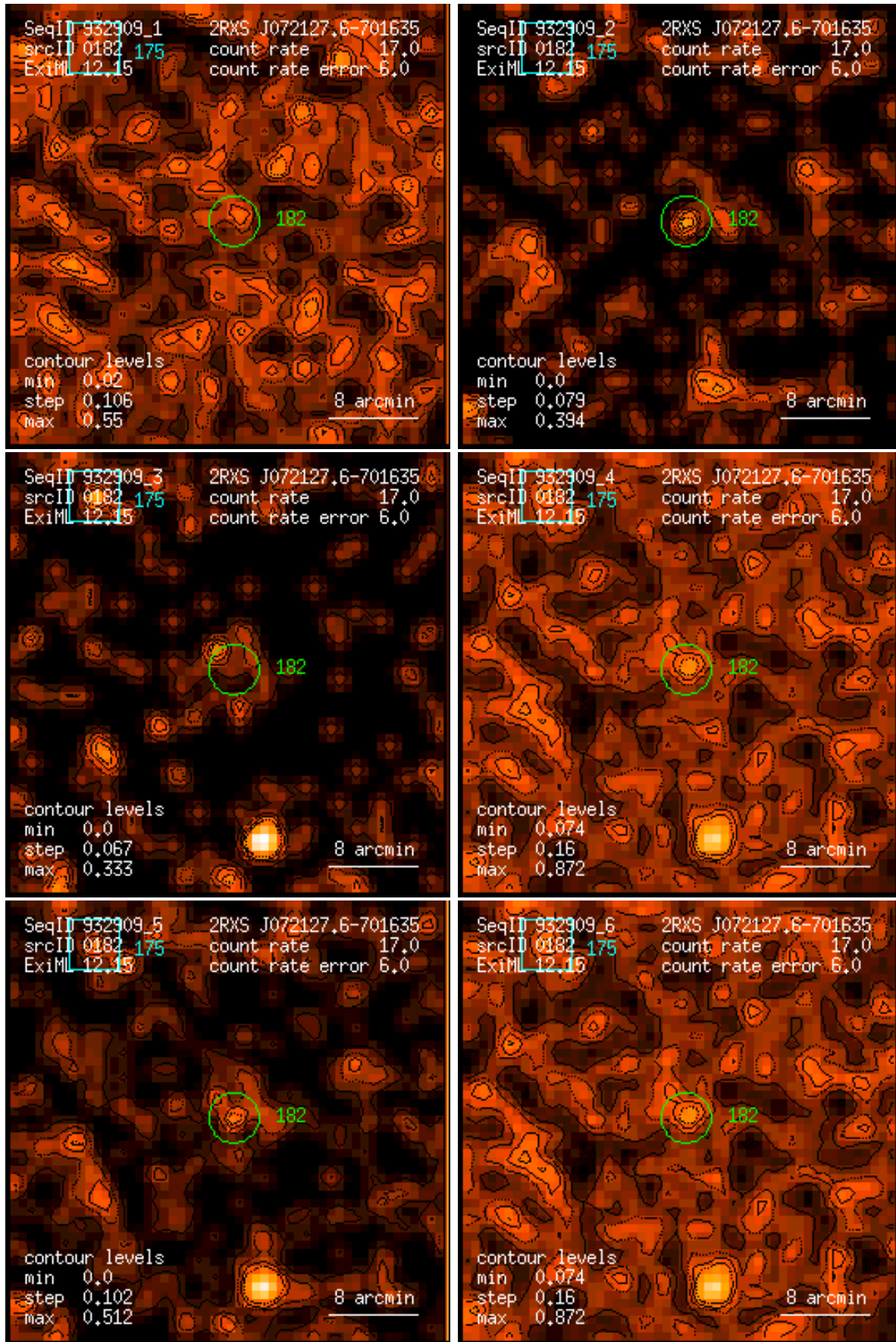
Figure 182: RASS 932909: detection 0182: band rate images, Gaussian filter: (1) PSPC channels 11 – 41, (2) 52 – 90, (3) 91 – 201, (4) 11 – 235, (5) 52 – 201, (6) 11 – 201. Broad band rates in counts/ks. Band rate contour levels in counts/ks/arcmin 2 .
