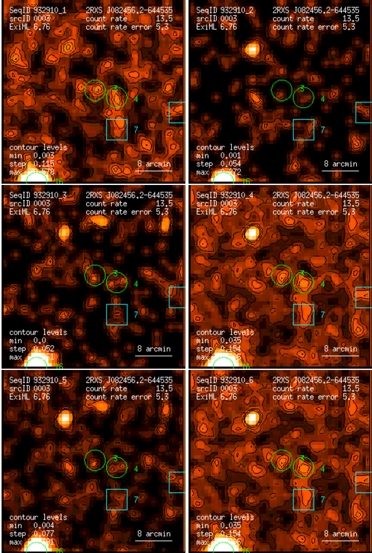
Figure 3: RASS 932910: detection 0003: band rate images, Gaussian filter: (1) PSPC channels 11 – 41, (2) 52 – 90, (3) 91 – 201, (4) 11 – 235, (5) 52 – 201, (6) 11 – 201. Broad band rates in counts/ks. Band rate contour levels in counts/ks/arcmin 2 .
