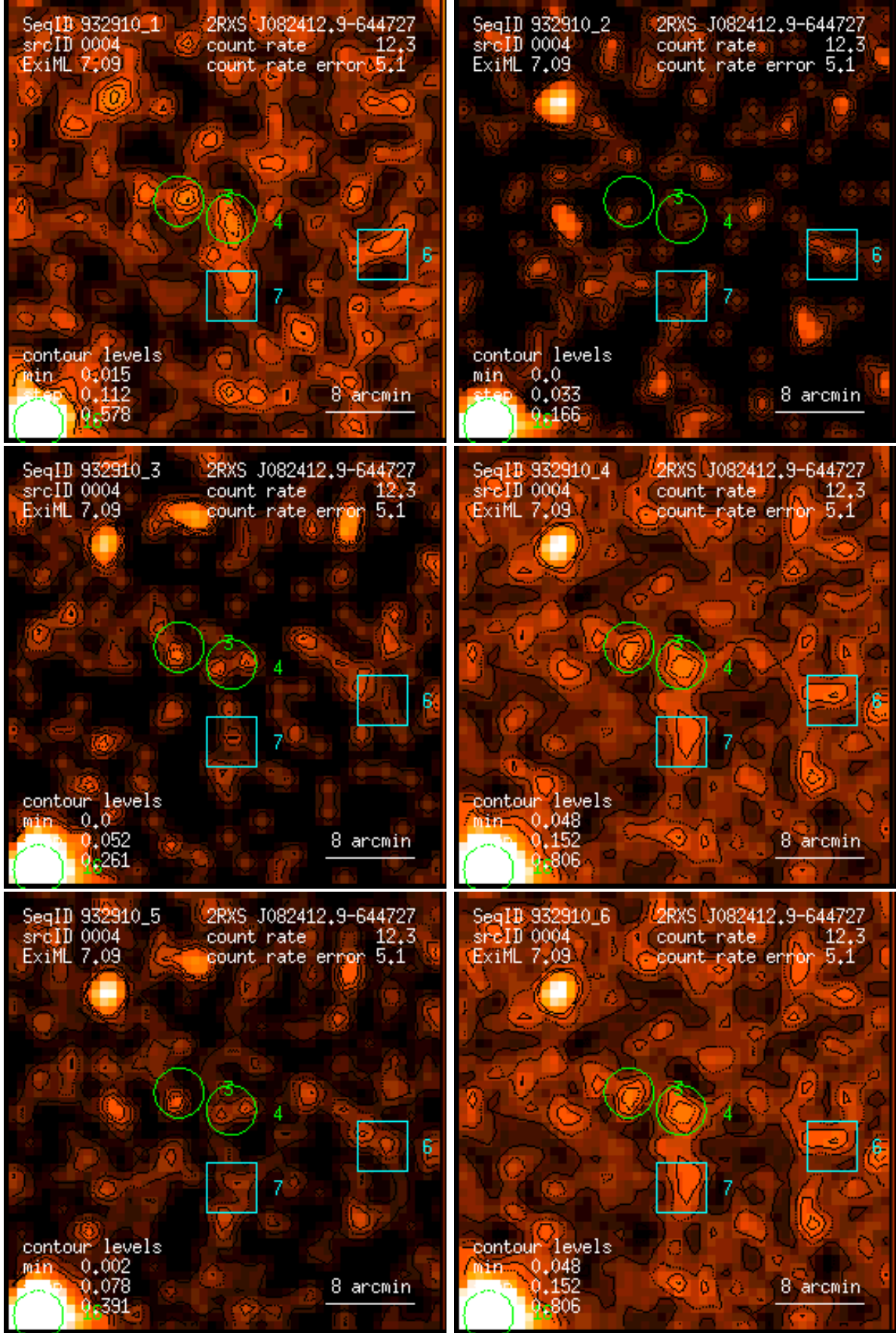
Figure 4: RASS 932910: detection 0004: band rate images, Gaussian filter: (1) PSPC channels 11 – 41, (2) 52 – 90, (3) 91 – 201, (4) 11 – 235, (5) 52 – 201, (6) 11 – 201. Broad band rates in counts/ks. Band rate contour levels in counts/ks/arcmin 2 .
