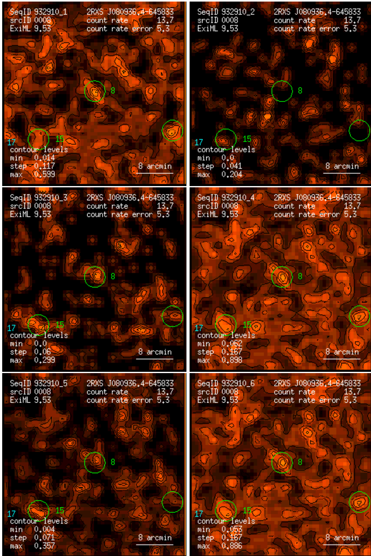
Figure 8: RASS 932910: detection 0008: band rate images, Gaussian filter: (1) PSPC channels 11 – 41, (2) 52 – 90, (3) 91 – 201, (4) 11 – 235, (5) 52 – 201, (6) 11 – 201. Broad band rates in counts/ks. Band rate contour levels in counts/ks/arcmin 2 .
