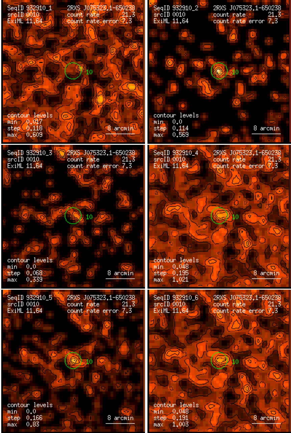
Figure 10: RASS 932910: detection 0010: band rate images, Gaussian filter: (1) PSPC channels 11 – 41, (2) 52 – 90, (3) 91 – 201, (4) 11 – 235, (5) 52 – 201, (6) 11 – 201. Broad band rates in counts/ks. Band rate contour levels in counts/ks/arcmin 2 .
