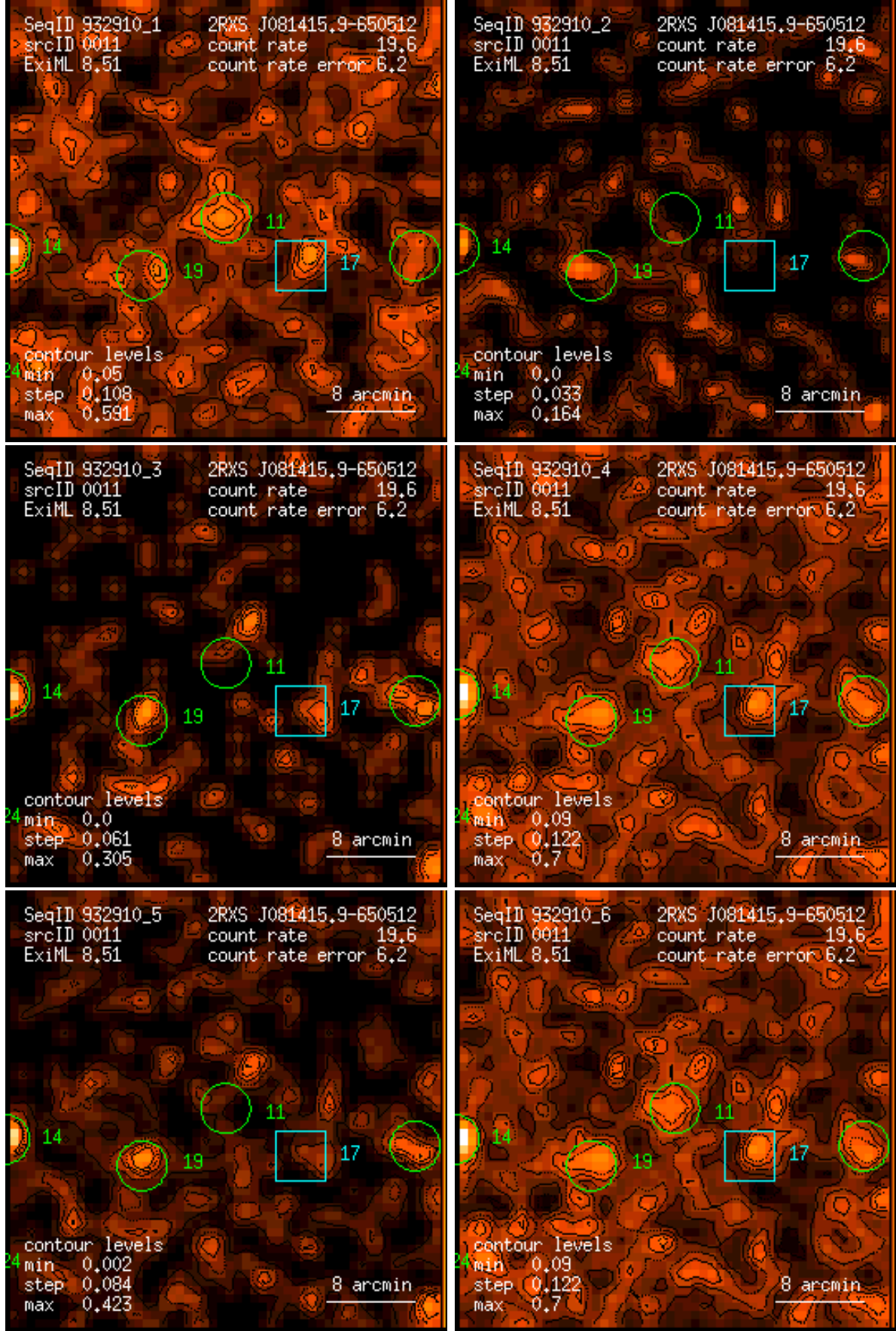
Figure 11: RASS 932910: detection 0011: band rate images, Gaussian filter: (1) PSPC channels 11 – 41, (2) 52 – 90, (3) 91 – 201, (4) 11 – 235, (5) 52 – 201, (6) 11 – 201. Broad band rates in counts/ks. Band rate contour levels in counts/ks/arcmin 2 .
