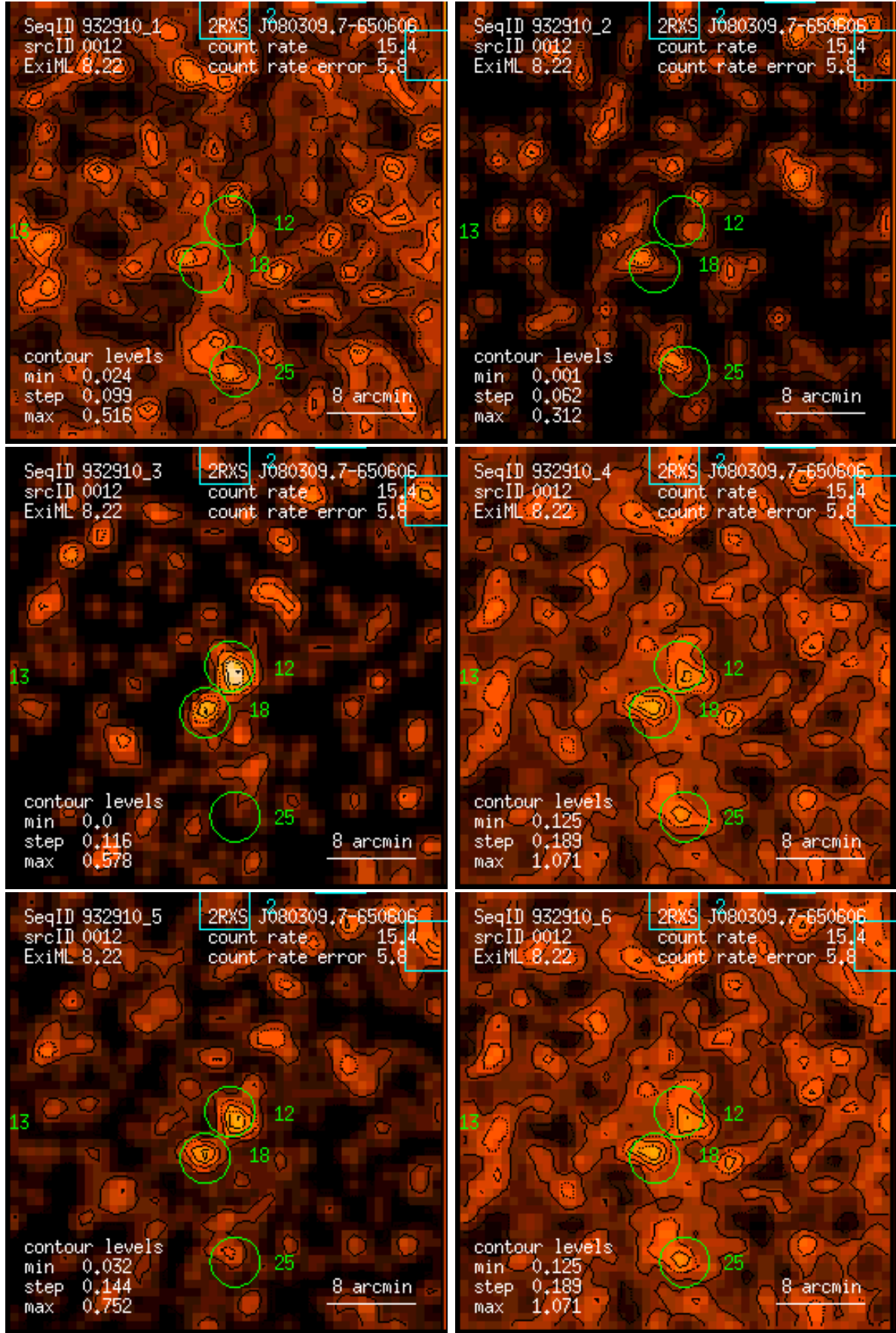
Figure 12: RASS 932910: detection 0012: band rate images, Gaussian filter: (1) PSPC channels 11 – 41, (2) 52 – 90, (3) 91 – 201, (4) 11 – 235, (5) 52 – 201, (6) 11 – 201. Broad band rates in counts/ks. Band rate contour levels in counts/ks/arcmin 2 .
