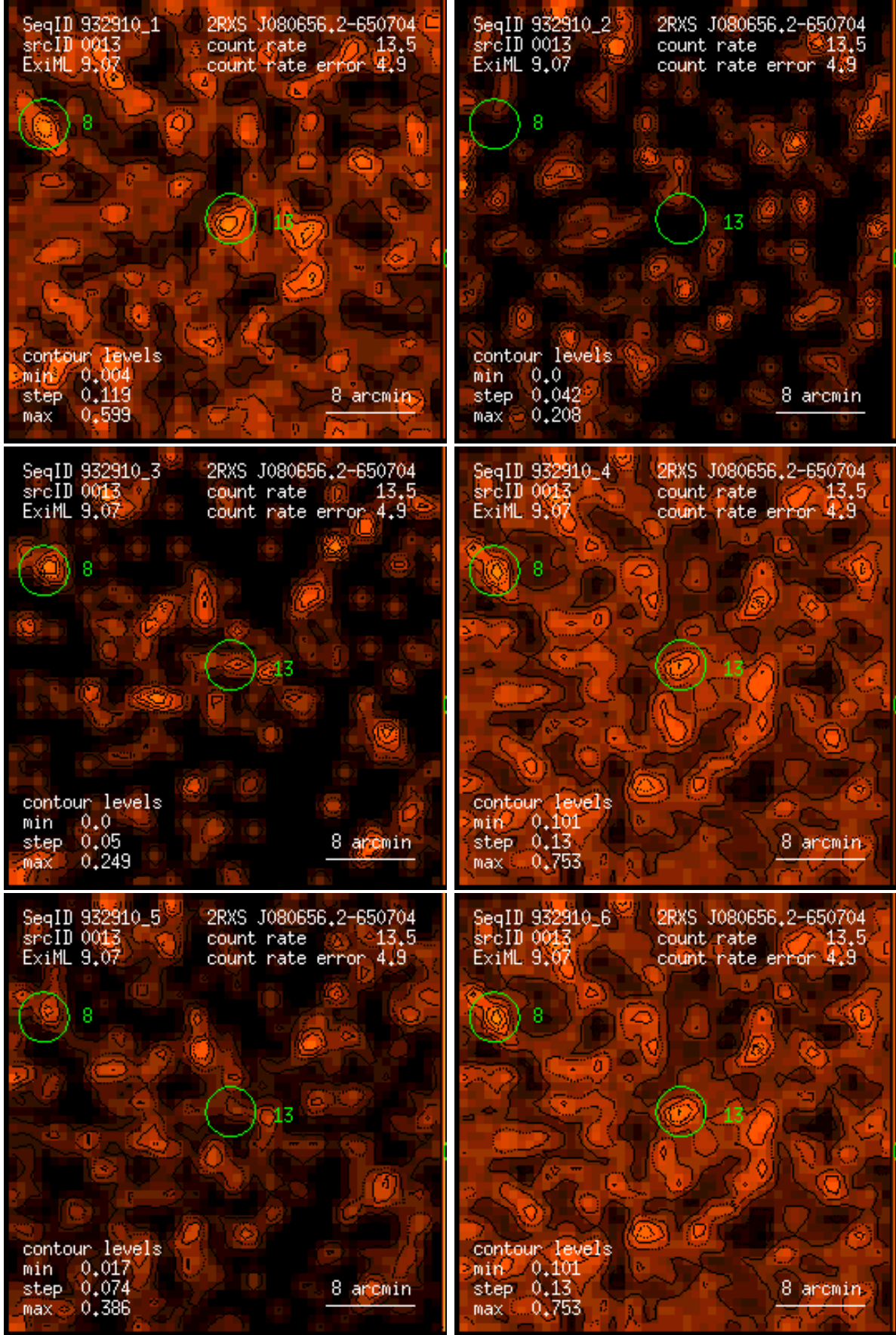
Figure 13: RASS 932910: detection 0013: band rate images, Gaussian filter: (1) PSPC channels 11 – 41, (2) 52 – 90, (3) 91 – 201, (4) 11 – 235, (5) 52 – 201, (6) 11 – 201. Broad band rates in counts/ks. Band rate contour levels in counts/ks/arcmin 2 .
