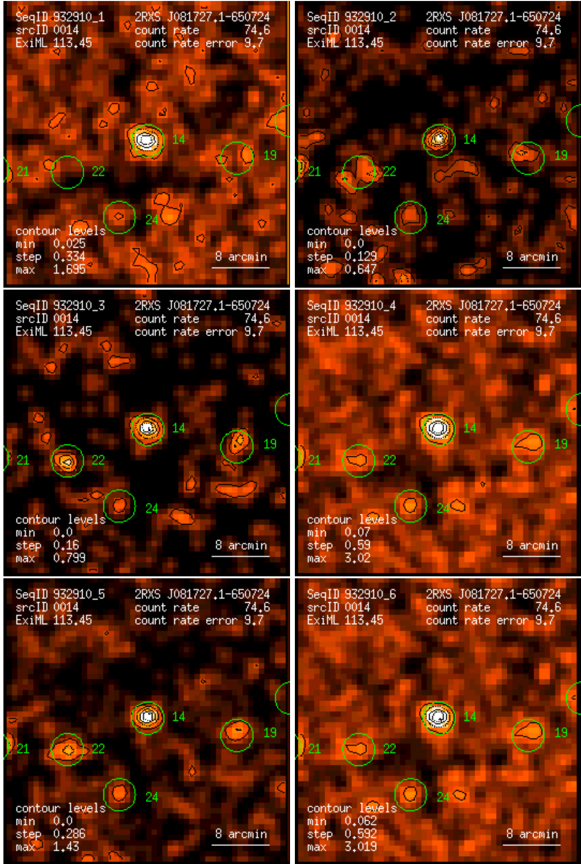
Figure 14: RASS 932910: detection 0014: band rate images, Gaussian filter: (1) PSPC channels 11 – 41, (2) 52 – 90, (3) 91 – 201, (4) 11 – 235, (5) 52 – 201, (6) 11 – 201. Broad band rates in counts/ks. Band rate contour levels in counts/ks/arcmin 2 .
