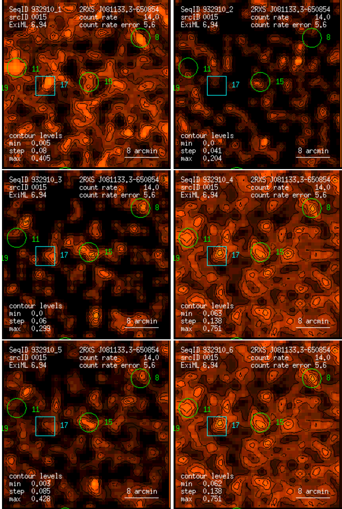
Figure 15: RASS 932910: detection 0015: band rate images, Gaussian filter: (1) PSPC channels 11 – 41, (2) 52 – 90, (3) 91 – 201, (4) 11 – 235, (5) 52 – 201, (6) 11 – 201. Broad band rates in counts/ks. Band rate contour levels in counts/ks/arcmin 2 .
