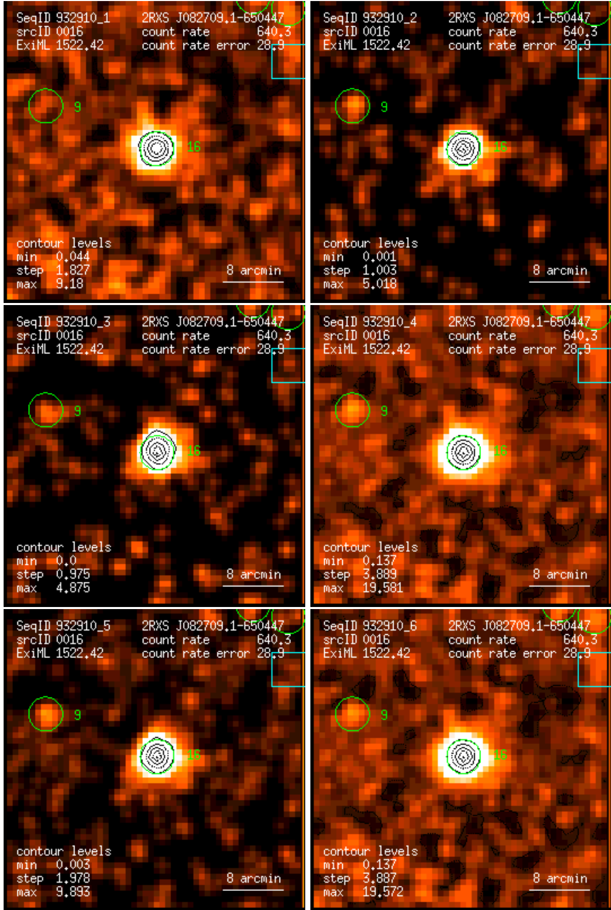
Figure 16: RASS 932910: detection 0016: band rate images, Gaussian filter: (1) PSPC channels 11 – 41, (2) 52 – 90, (3) 91 – 201, (4) 11 – 235, (5) 52 – 201, (6) 11 – 201. Broad band rates in counts/ks. Band rate contour levels in counts/ks/arcmin 2 .
