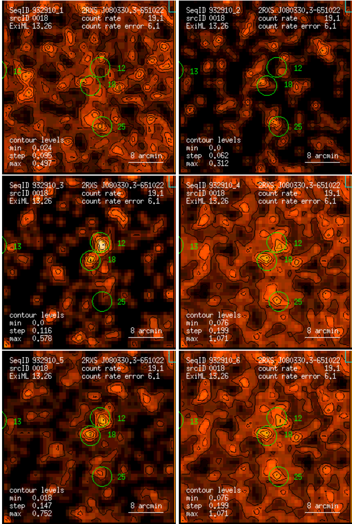
Figure 18: RASS 932910: detection 0018: band rate images, Gaussian filter: (1) PSPC channels 11 – 41, (2) 52 – 90, (3) 91 – 201, (4) 11 – 235, (5) 52 – 201, (6) 11 – 201. Broad band rates in counts/ks. Band rate contour levels in counts/ks/arcmin 2 .
