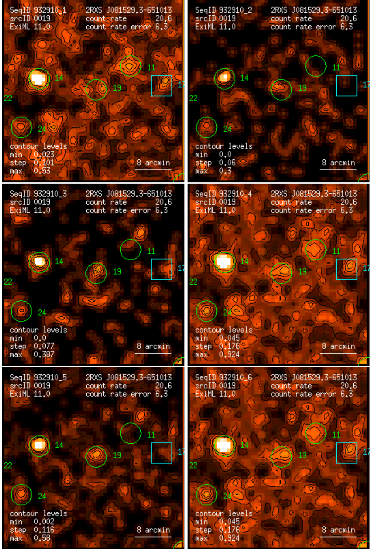
Figure 19: RASS 932910: detection 0019: band rate images, Gaussian filter: (1) PSPC channels 11 – 41, (2) 52 – 90, (3) 91 – 201, (4) 11 – 235, (5) 52 – 201, (6) 11 – 201. Broad band rates in counts/ks. Band rate contour levels in counts/ks/arcmin 2 .
