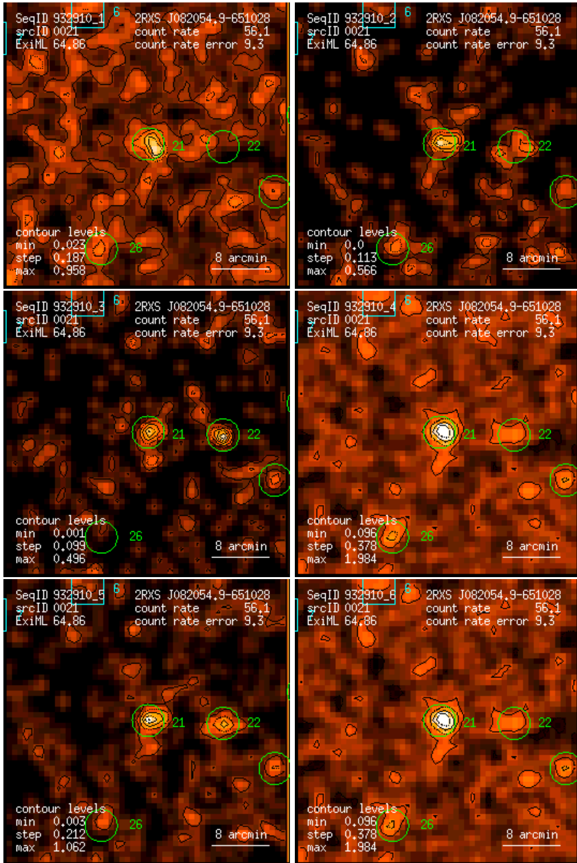
Figure 21: RASS 932910: detection 0021: band rate images, Gaussian filter: (1) PSPC channels 11 – 41, (2) 52 – 90, (3) 91 – 201, (4) 11 – 235, (5) 52 – 201, (6) 11 – 201. Broad band rates in counts/ks. Band rate contour levels in counts/ks/arcmin 2 .
