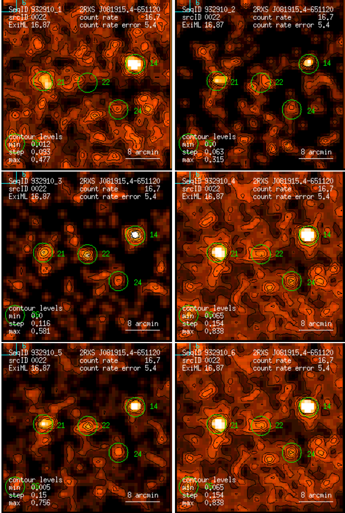
Figure 22: RASS 932910: detection 0022: band rate images, Gaussian filter: (1) PSPC channels 11 – 41, (2) 52 – 90, (3) 91 – 201, (4) 11 – 235, (5) 52 – 201, (6) 11 – 201. Broad band rates in counts/ks. Band rate contour levels in counts/ks/arcmin 2 .
