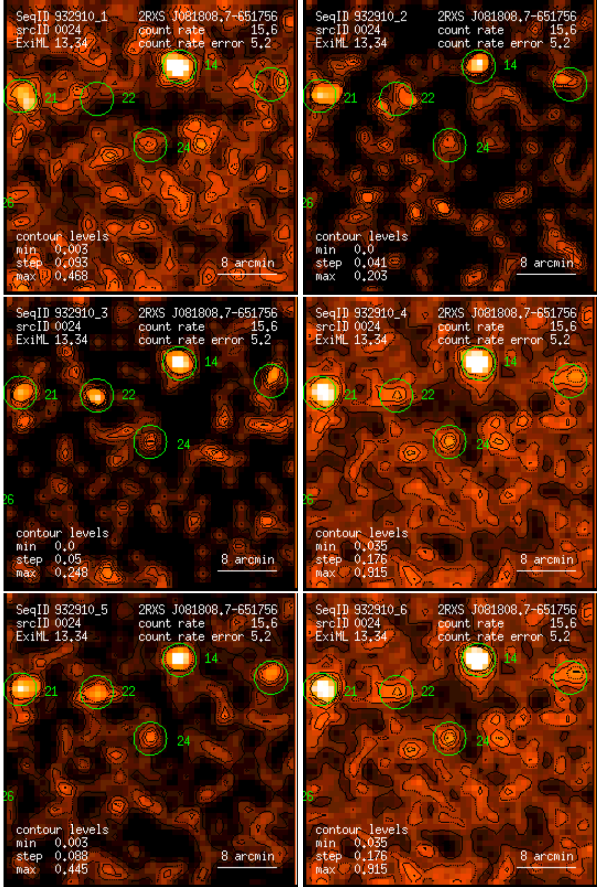
Figure 24: RASS 932910: detection 0024: band rate images, Gaussian filter: (1) PSPC channels 11 – 41, (2) 52 – 90, (3) 91 – 201, (4) 11 – 235, (5) 52 – 201, (6) 11 – 201. Broad band rates in counts/ks. Band rate contour levels in counts/ks/arcmin 2 .
