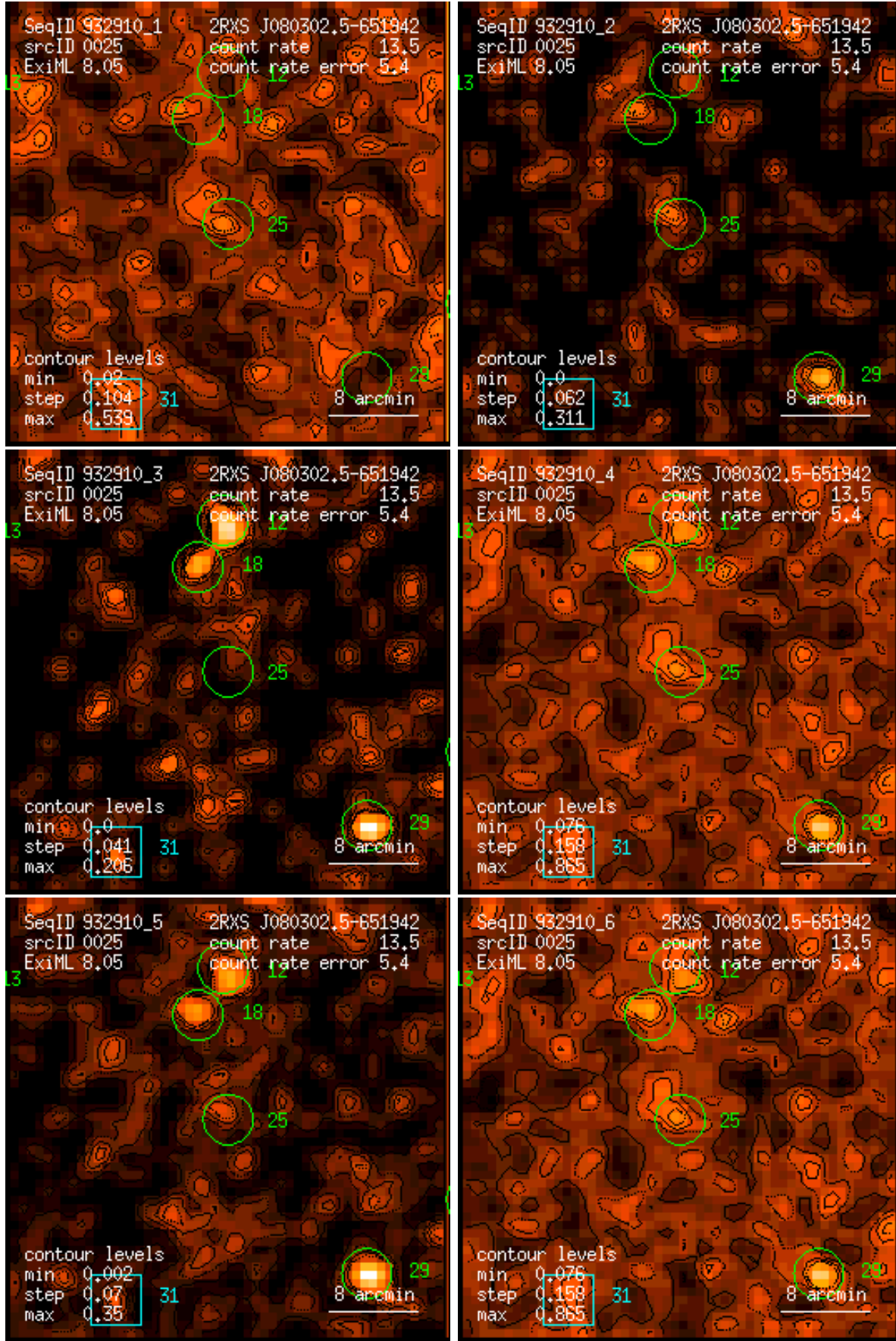
Figure 25: RASS 932910: detection 0025: band rate images, Gaussian filter: (1) PSPC channels 11 – 41, (2) 52 – 90, (3) 91 – 201, (4) 11 – 235, (5) 52 – 201, (6) 11 – 201. Broad band rates in counts/ks. Band rate contour levels in counts/ks/arcmin 2 .
