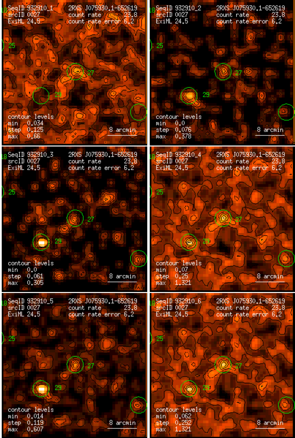
Figure 27: RASS 932910: detection 0027: band rate images, Gaussian filter: (1) PSPC channels 11 – 41, (2) 52 – 90, (3) 91 – 201, (4) 11 – 235, (5) 52 – 201, (6) 11 – 201. Broad band rates in counts/ks. Band rate contour levels in counts/ks/arcmin 2 .
