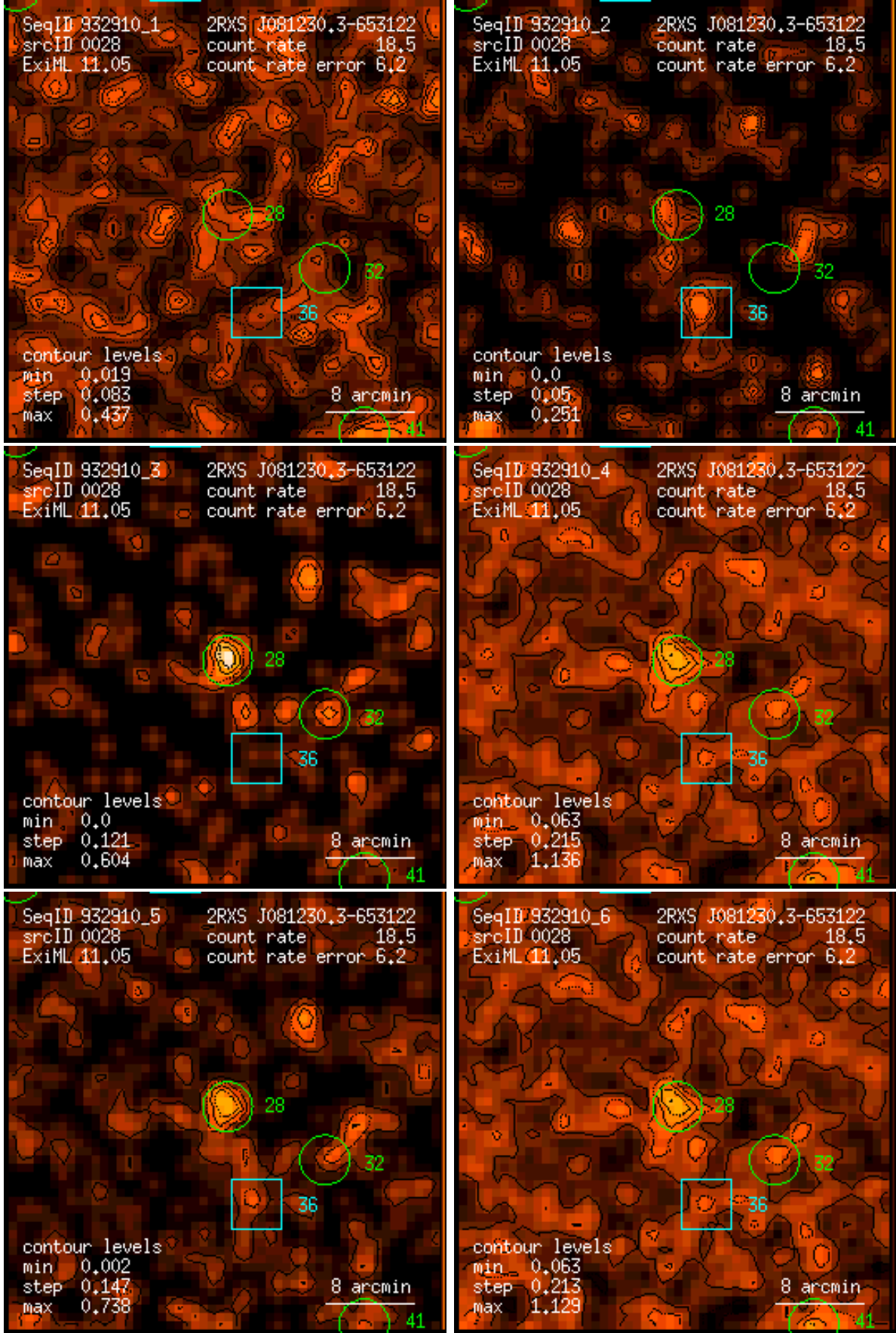
Figure 28: RASS 932910: detection 0028: band rate images, Gaussian filter: (1) PSPC channels 11 – 41, (2) 52 – 90, (3) 91 – 201, (4) 11 – 235, (5) 52 – 201, (6) 11 – 201. Broad band rates in counts/ks. Band rate contour levels in counts/ks/arcmin 2 .
