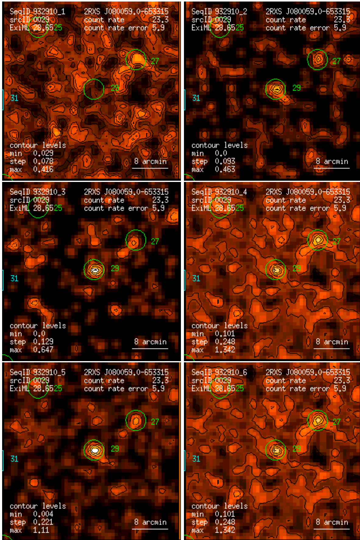
Figure 29: RASS 932910: detection 0029: band rate images, Gaussian filter: (1) PSPC channels 11 – 41, (2) 52 – 90, (3) 91 – 201, (4) 11 – 235, (5) 52 – 201, (6) 11 – 201. Broad band rates in counts/ks. Band rate contour levels in counts/ks/arcmin 2 .
