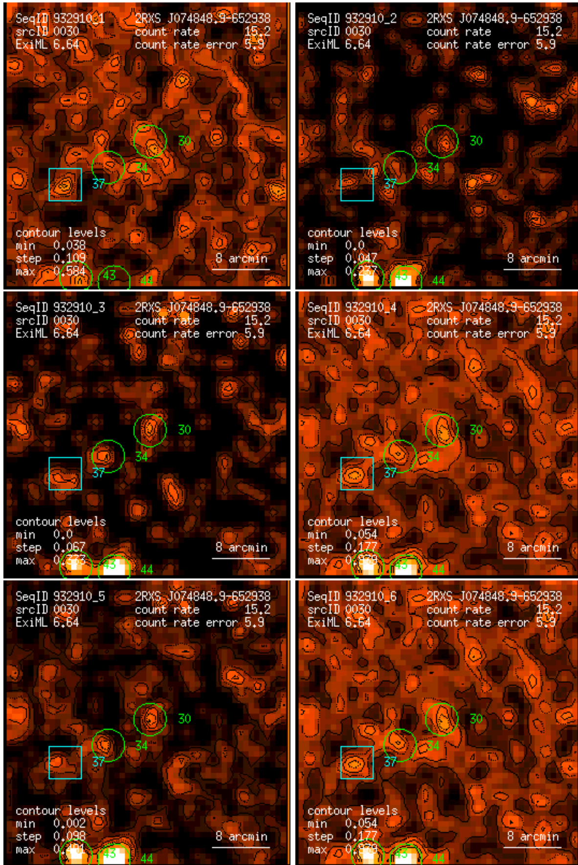
Figure 30: RASS 932910: detection 0030: band rate images, Gaussian filter: (1) PSPC channels 11 – 41, (2) 52 – 90, (3) 91 – 201, (4) 11 – 235, (5) 52 – 201, (6) 11 – 201. Broad band rates in counts/ks. Band rate contour levels in counts/ks/arcmin 2 .
