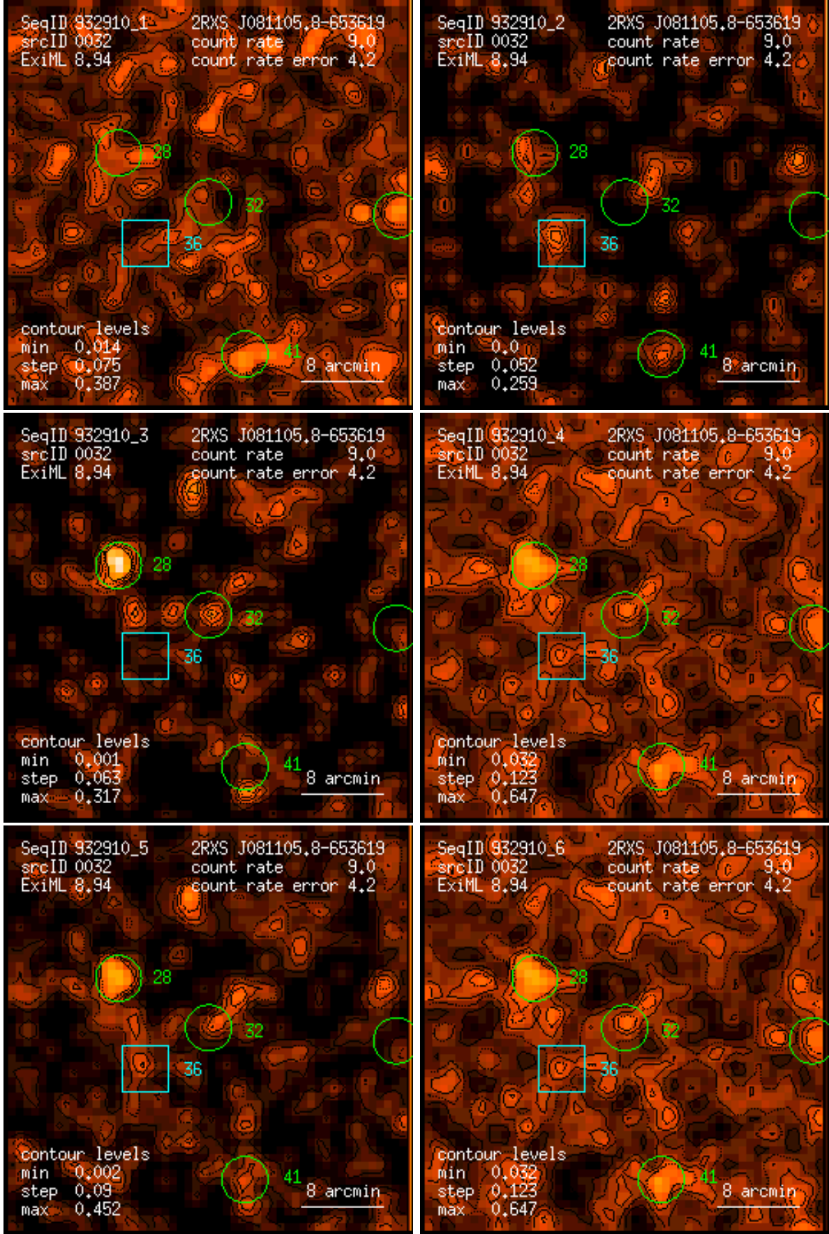
Figure 32: RASS 932910: detection 0032: band rate images, Gaussian filter: (1) PSPC channels 11 – 41, (2) 52 – 90, (3) 91 – 201, (4) 11 – 235, (5) 52 – 201, (6) 11 – 201. Broad band rates in counts/ks. Band rate contour levels in counts/ks/arcmin 2 .
