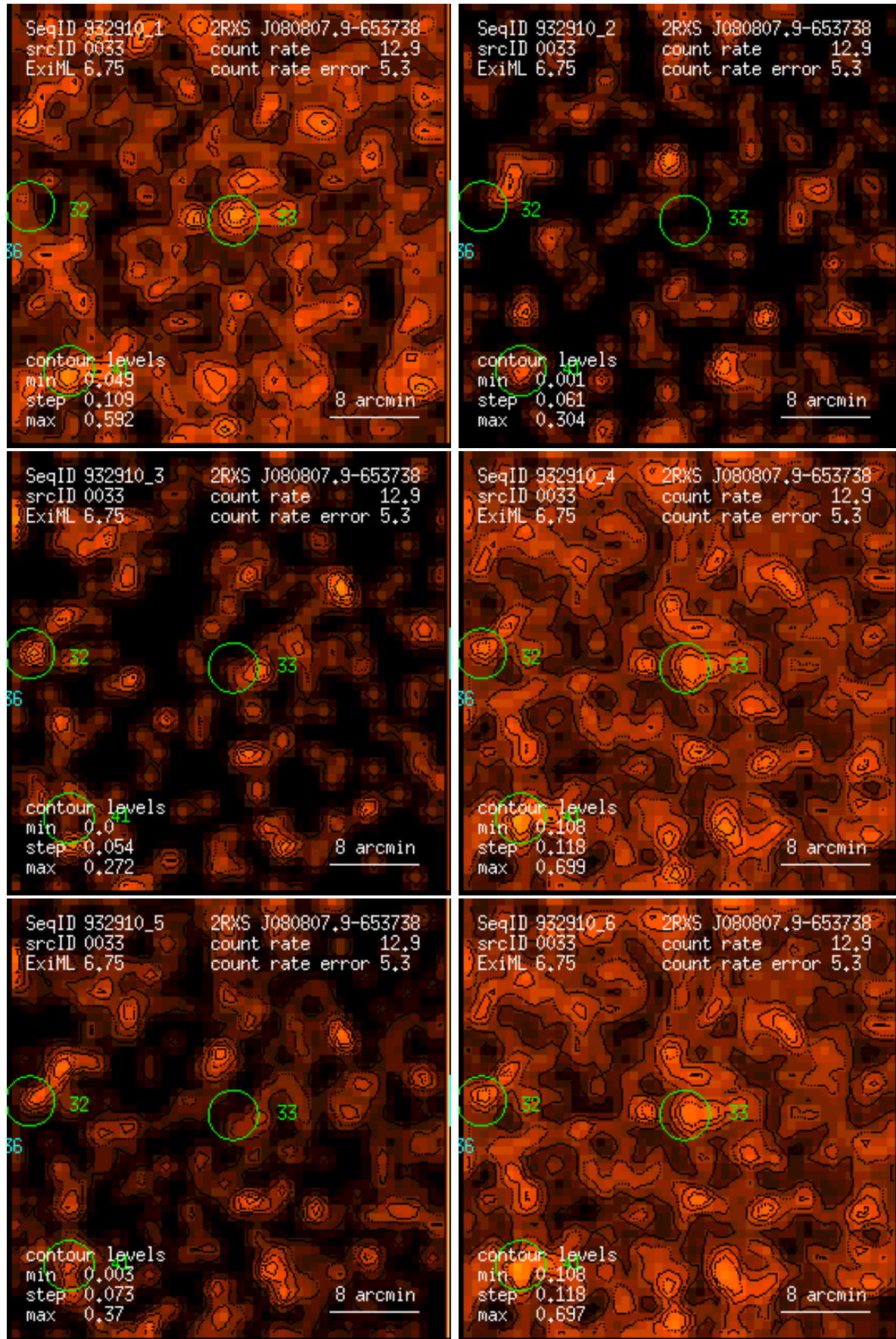
Figure 33: RASS 932910: detection 0033: band rate images, Gaussian filter: (1) PSPC channels 11 – 41, (2) 52 – 90, (3) 91 – 201, (4) 11 – 235, (5) 52 – 201, (6) 11 – 201. Broad band rates in counts/ks. Band rate contour levels in counts/ks/arcmin 2 .
