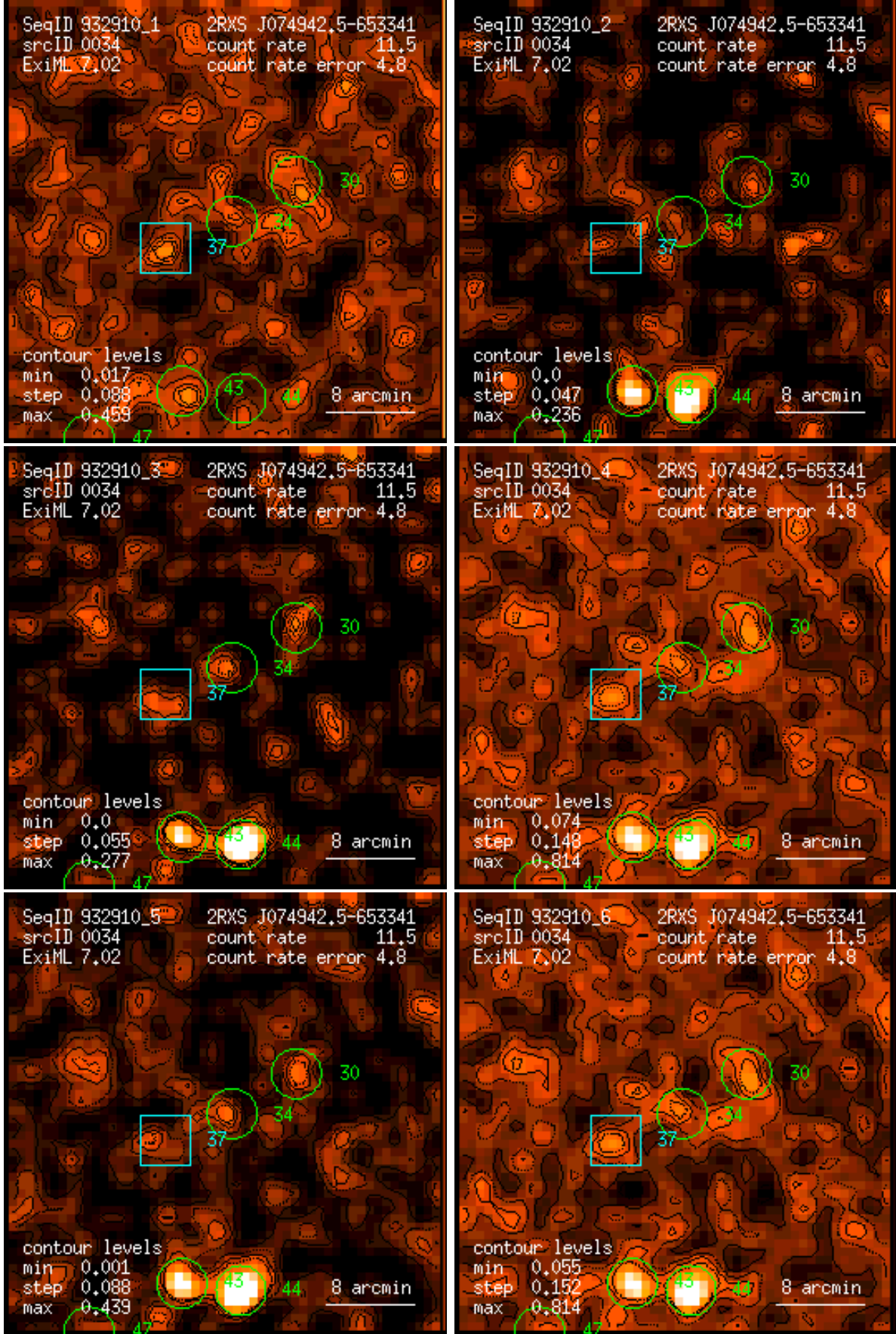
Figure 34: RASS 932910: detection 0034: band rate images, Gaussian filter: (1) PSPC channels 11 – 41, (2) 52 – 90, (3) 91 – 201, (4) 11 – 235, (5) 52 – 201, (6) 11 – 201. Broad band rates in counts/ks. Band rate contour levels in counts/ks/arcmin 2 .
