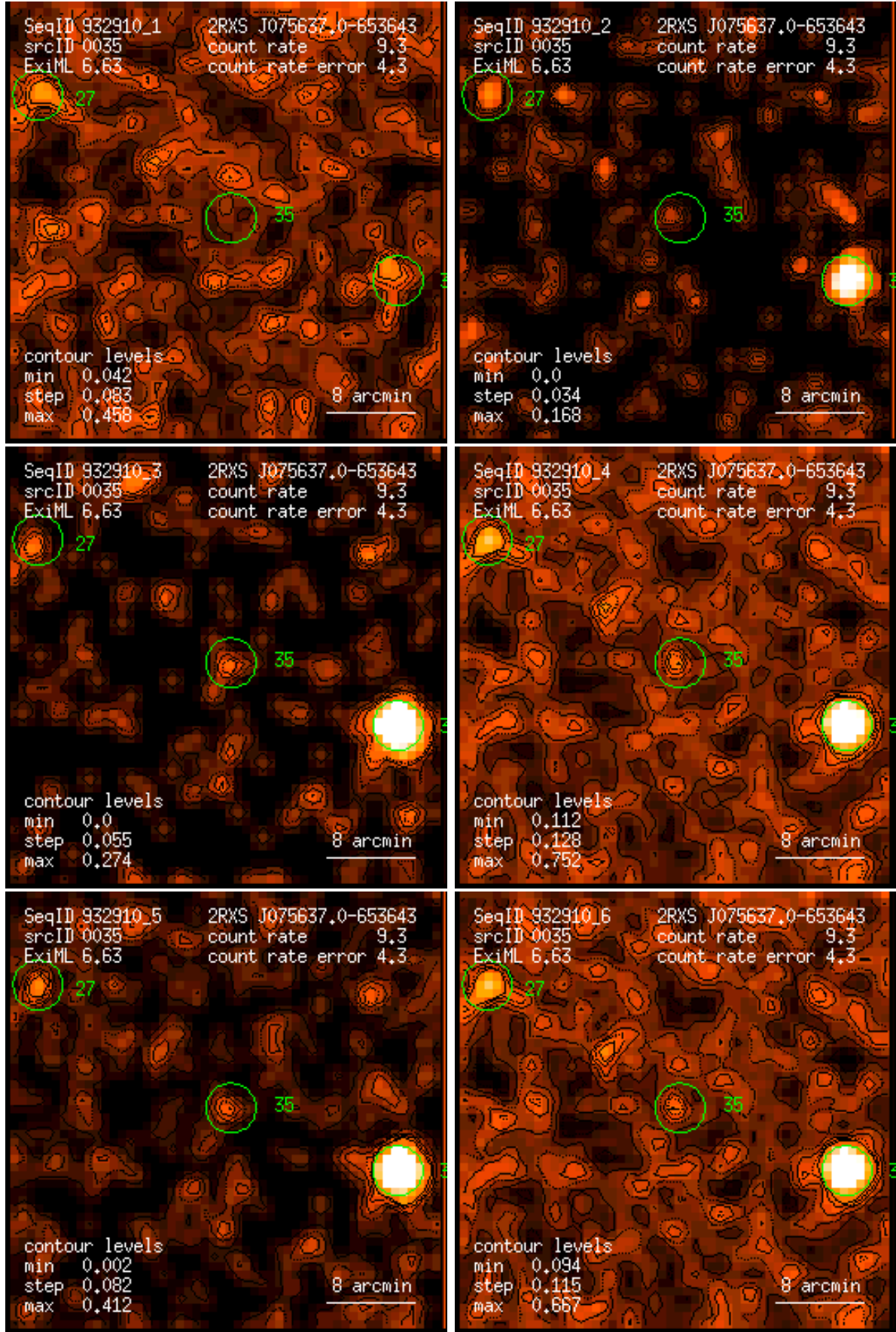
Figure 35: RASS 932910: detection 0035: band rate images, Gaussian filter: (1) PSPC channels 11 – 41, (2) 52 – 90, (3) 91 – 201, (4) 11 – 235, (5) 52 – 201, (6) 11 – 201. Broad band rates in counts/ks. Band rate contour levels in counts/ks/arcmin 2 .
