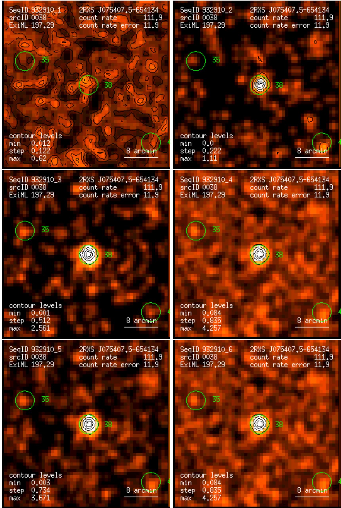
Figure 38: RASS 932910: detection 0038: band rate images, Gaussian filter: (1) PSPC channels 11 – 41, (2) 52 – 90, (3) 91 – 201, (4) 11 – 235, (5) 52 – 201, (6) 11 – 201. Broad band rates in counts/ks. Band rate contour levels in counts/ks/arcmin 2 .
