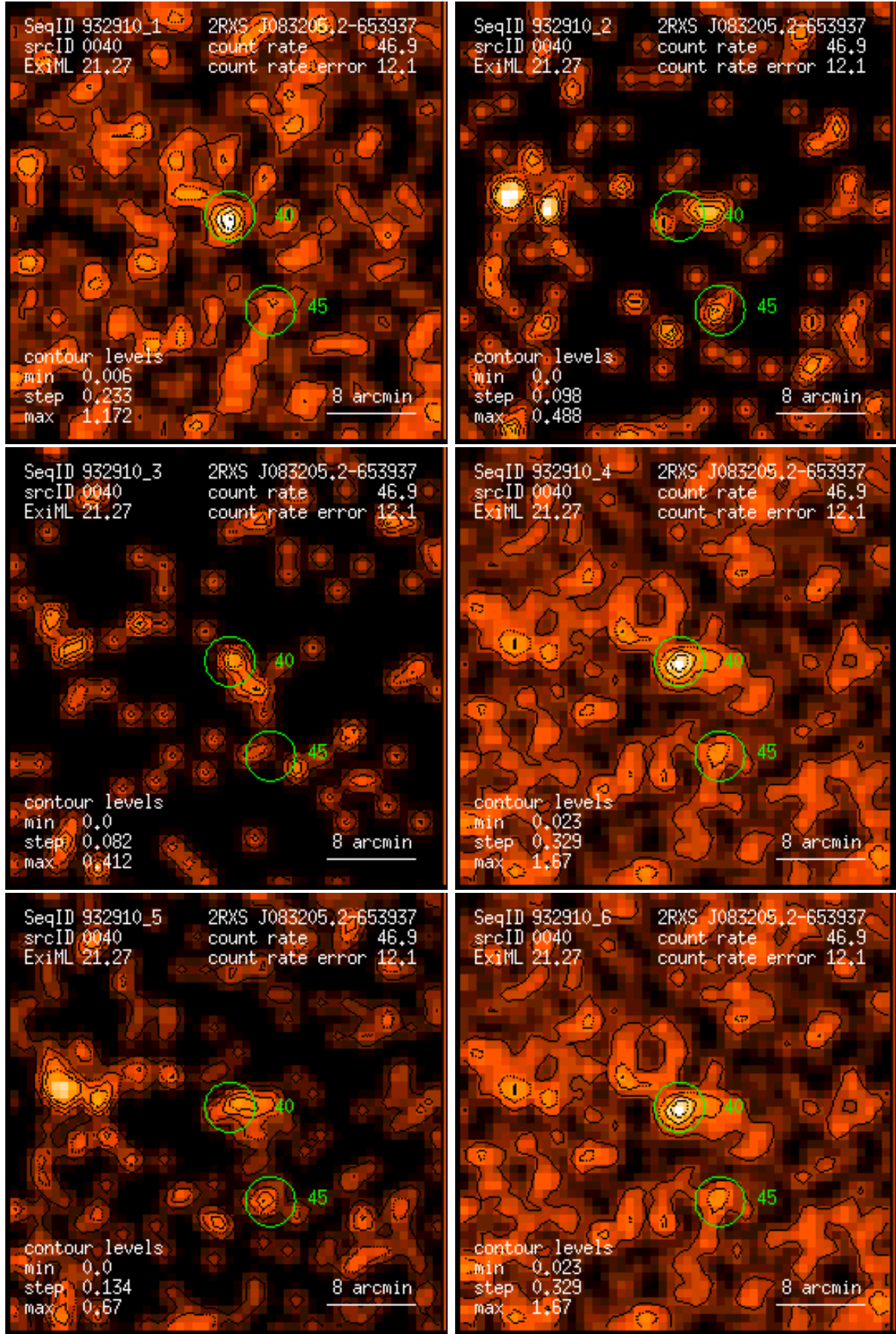
Figure 40: RASS 932910: detection 0040: band rate images, Gaussian filter: (1) PSPP channels 11 – 41, (2) 52 – 90, (3) 91 – 201, (4) 11 – 235, (5) 52 – 201, (6) 11 – 201. Broad band rates in counts/ks. Band rate contour levels in counts/ks/arcmin 2 .
