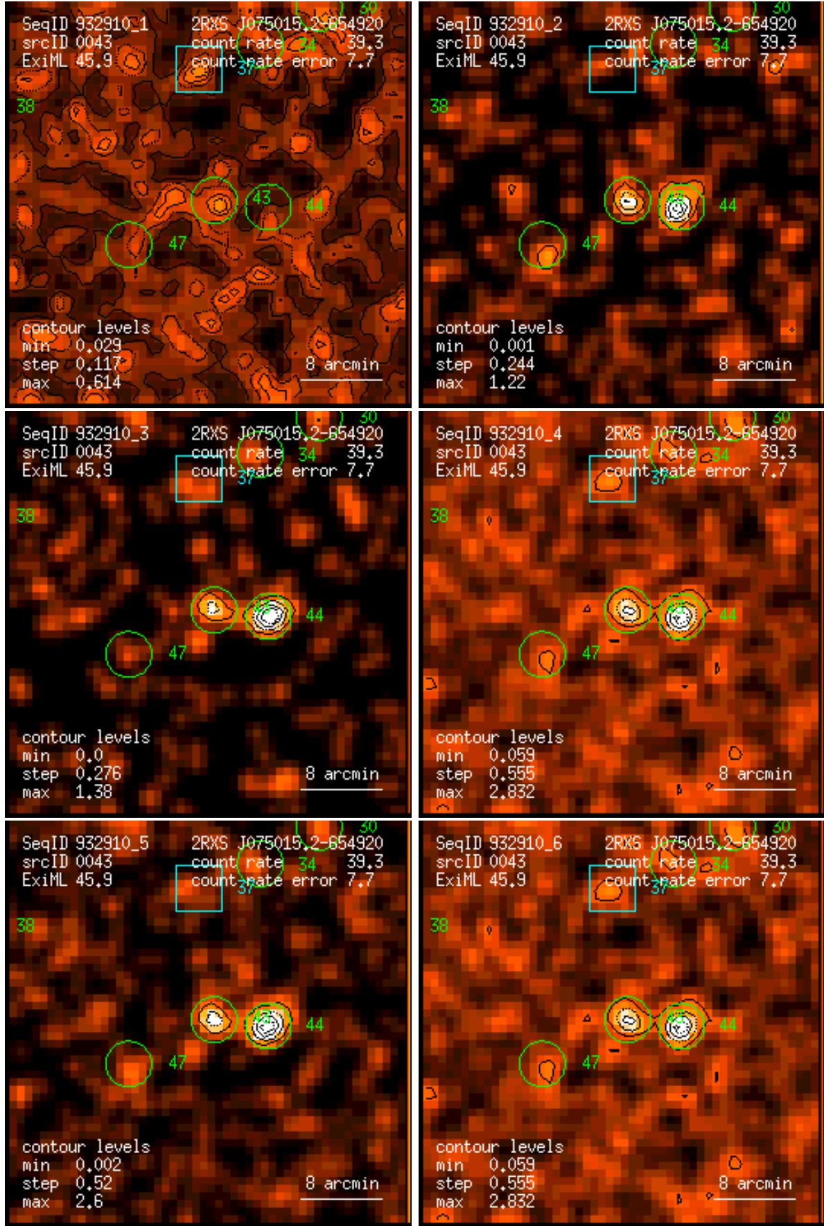
Figure 43: RASS 932910: detection 0043: band rate images, Gaussian filter: (1) PSPC channels 11 – 41, (2) 52 – 90, (3) 91 – 201, (4) 11 – 235, (5) 52 – 201, (6) 11 – 201. Broad band rates in counts/ks. Band rate contour levels in counts/ks/arcmin 2 .
