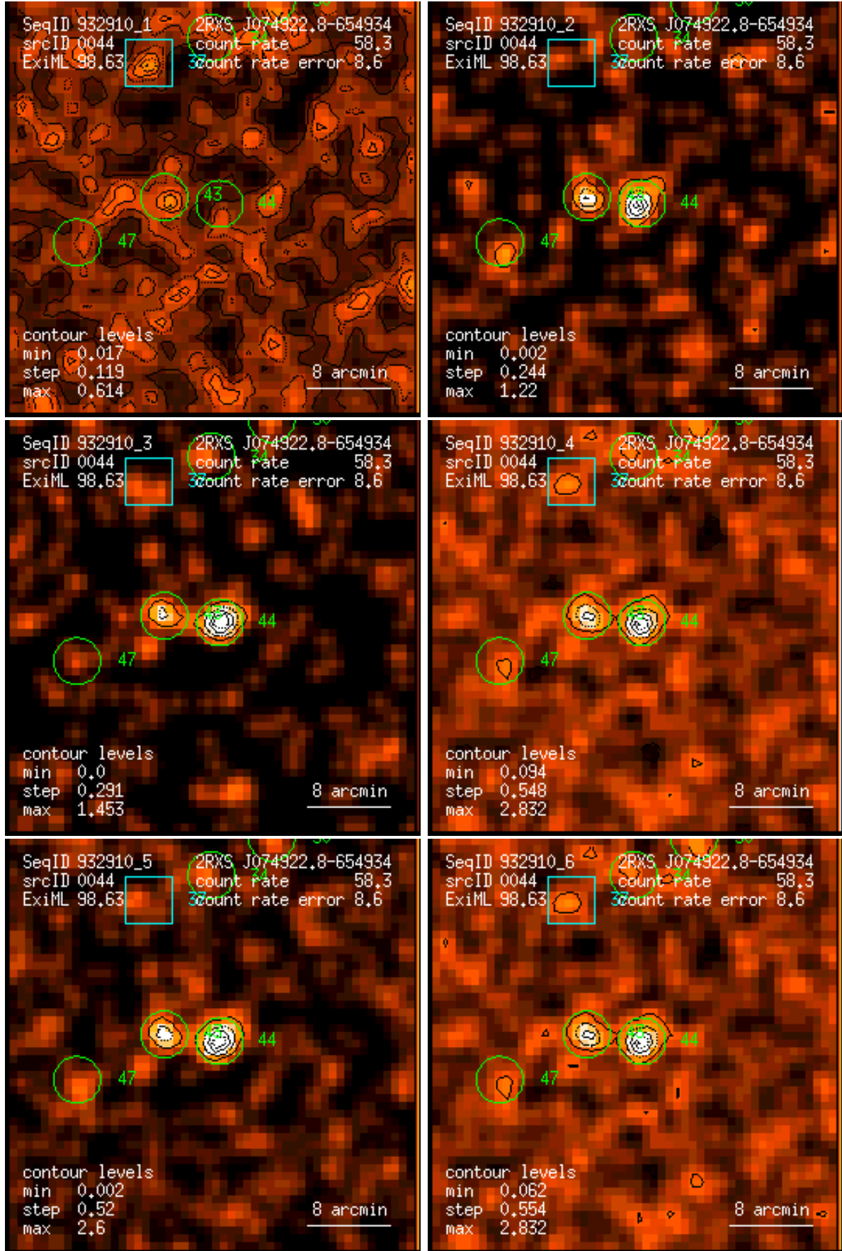
Figure 44: RASS 932910: detection 0044: band rate images, Gaussian filter: (1) PSPC channels 11 – 41, (2) 52 – 90, (3) 91 – 201, (4) 11 – 235, (5) 52 – 201, (6) 11 – 201. Broad band rates in counts/ks. Band rate contour levels in counts/ks/arcmin 2 .
