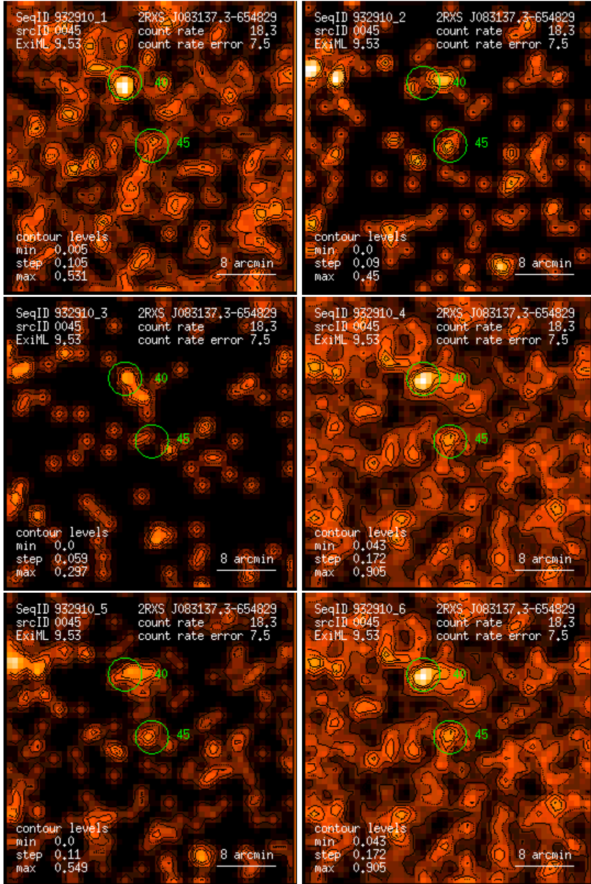
Figure 45: RASS 932910: detection 0045: band rate images, Gaussian filter: (1) PSPC channels 11 – 41, (2) 52 – 90, (3) 91 – 201, (4) 11 – 235, (5) 52 – 201, (6) 11 – 201. Broad band rates in counts/ks. Band rate contour levels in counts/ks/arcmin 2 .
