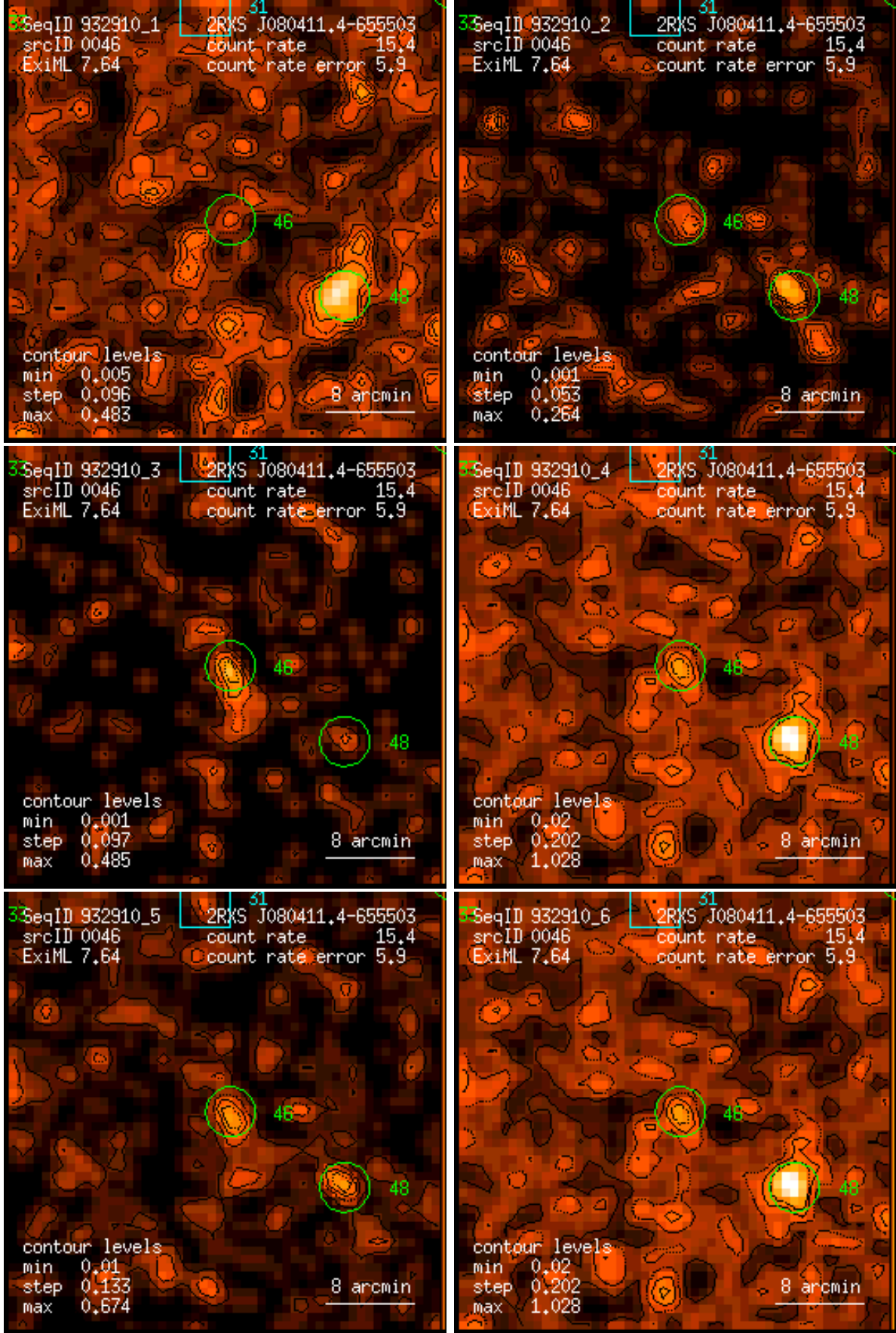
Figure 46: RASS 932910: detection 0046: band rate images, Gaussian filter: (1) PSPC channels 11 – 41, (2) 52 – 90, (3) 91 – 201, (4) 11 – 235, (5) 52 – 201, (6) 11 – 201. Broad band rates in counts/ks. Band rate contour levels in counts/ks/arcmin 2 .
