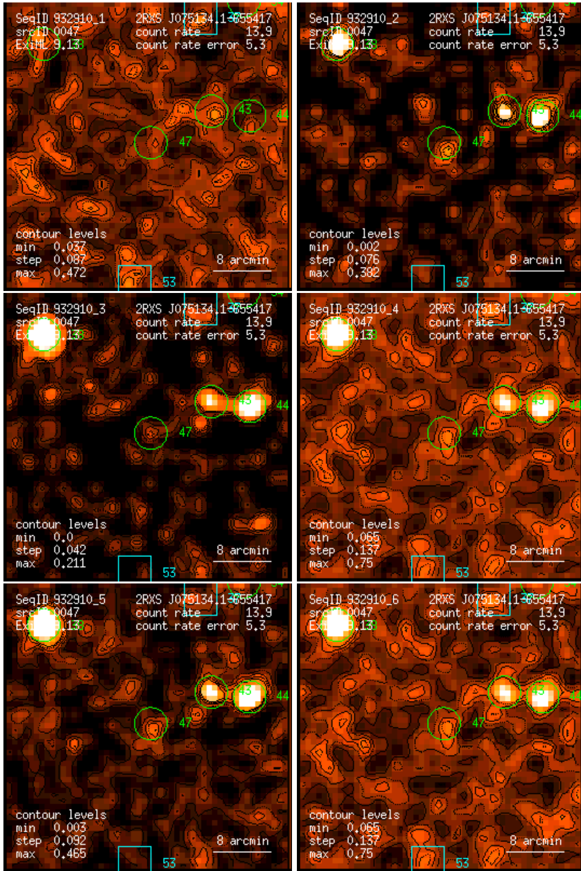
Figure 47: RASS 932910: detection 0047: band rate images, Gaussian filter: (1) PSPC channels 11 – 41, (2) 52 – 90, (3) 91 – 201, (4) 11 – 235, (5) 52 – 201, (6) 11 – 201. Broad band rates in counts/ks. Band rate contour levels in counts/ks/arcmin 2 .
