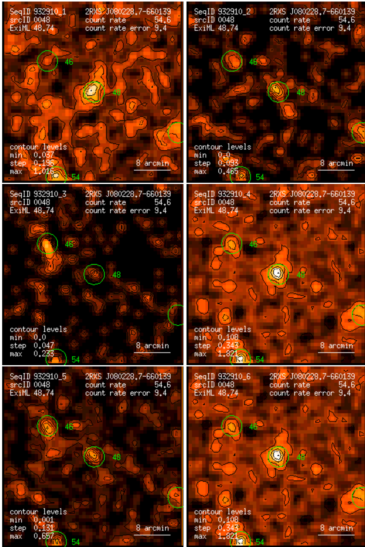
Figure 48: RASS 932910: detection 0048: band rate images, Gaussian filter: (1) PSPC channels 11 – 41, (2) 52 – 90, (3) 91 – 201, (4) 11 – 235, (5) 52 – 201, (6) 11 – 201. Broad band rates in counts/ks. Band rate contour levels in counts/ks/arcmin 2 .
