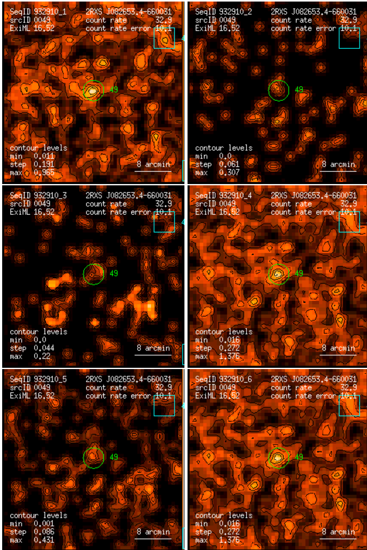
Figure 49: RASS 932910: detection 0049: band rate images, Gaussian filter: (1) PSPC channels 11 – 41, (2) 52 – 90, (3) 91 – 201, (4) 11 – 235, (5) 52 – 201, (6) 11 – 201. Broad band rates in counts/ks. Band rate contour levels in counts/ks/arcmin 2 .
