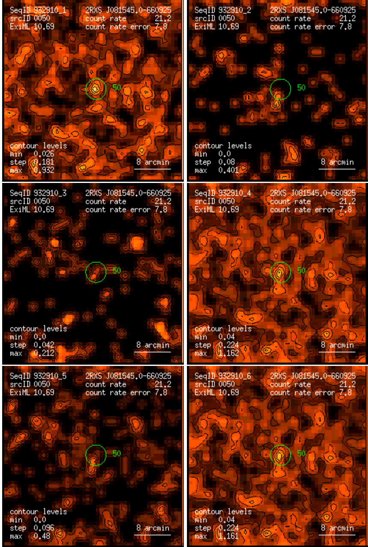
Figure 50: RASS 932910: detection 0050: band rate images, Gaussian filter: (1) PSPC channels 11 – 41, (2) 52 – 90, (3) 91 – 201, (4) 11 – 235, (5) 52 – 201, (6) 11 – 201. Broad band rates in counts/ks. Band rate contour levels in counts/ks/arcmin 2 .
