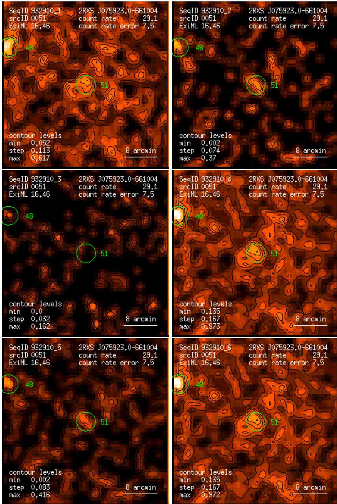
Figure 51: RASS 932910: detection 0051: band rate images, Gaussian filter: (1) PSPC channels 11 – 41, (2) 52 – 90, (3) 91 – 201, (4) 11 – 235, (5) 52 – 201, (6) 11 – 201. Broad band rates in counts/ks. Band rate contour levels in counts/ks/arcmin 2 .
