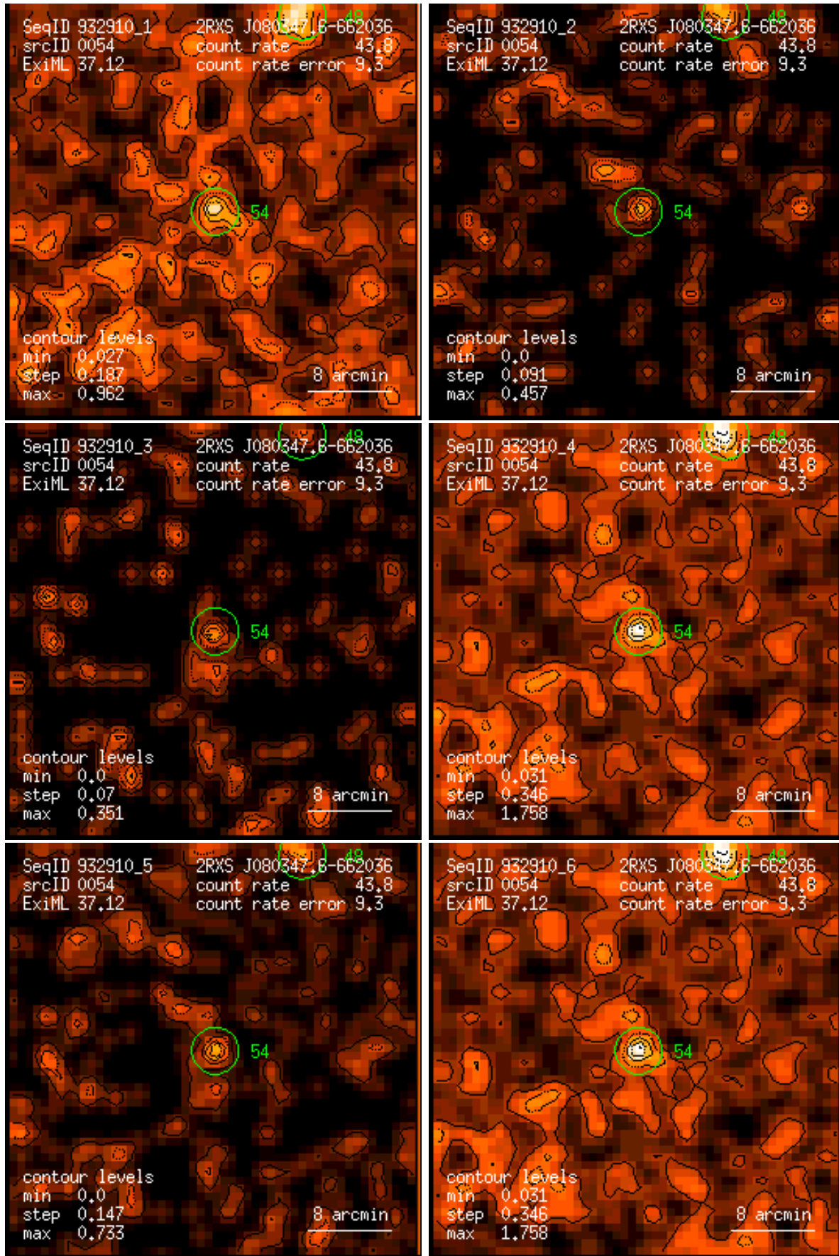
Figure 54: RASS 932910: detection 0054: band rate images, Gaussian filter: (1) PSPC channels 11 – 41, (2) 52 – 90, (3) 91 – 201, (4) 11 – 235, (5) 52 – 201, (6) 11 – 201. Broad band rates in counts/ks. Band rate contour levels in counts/ks/arcmin 2 .
