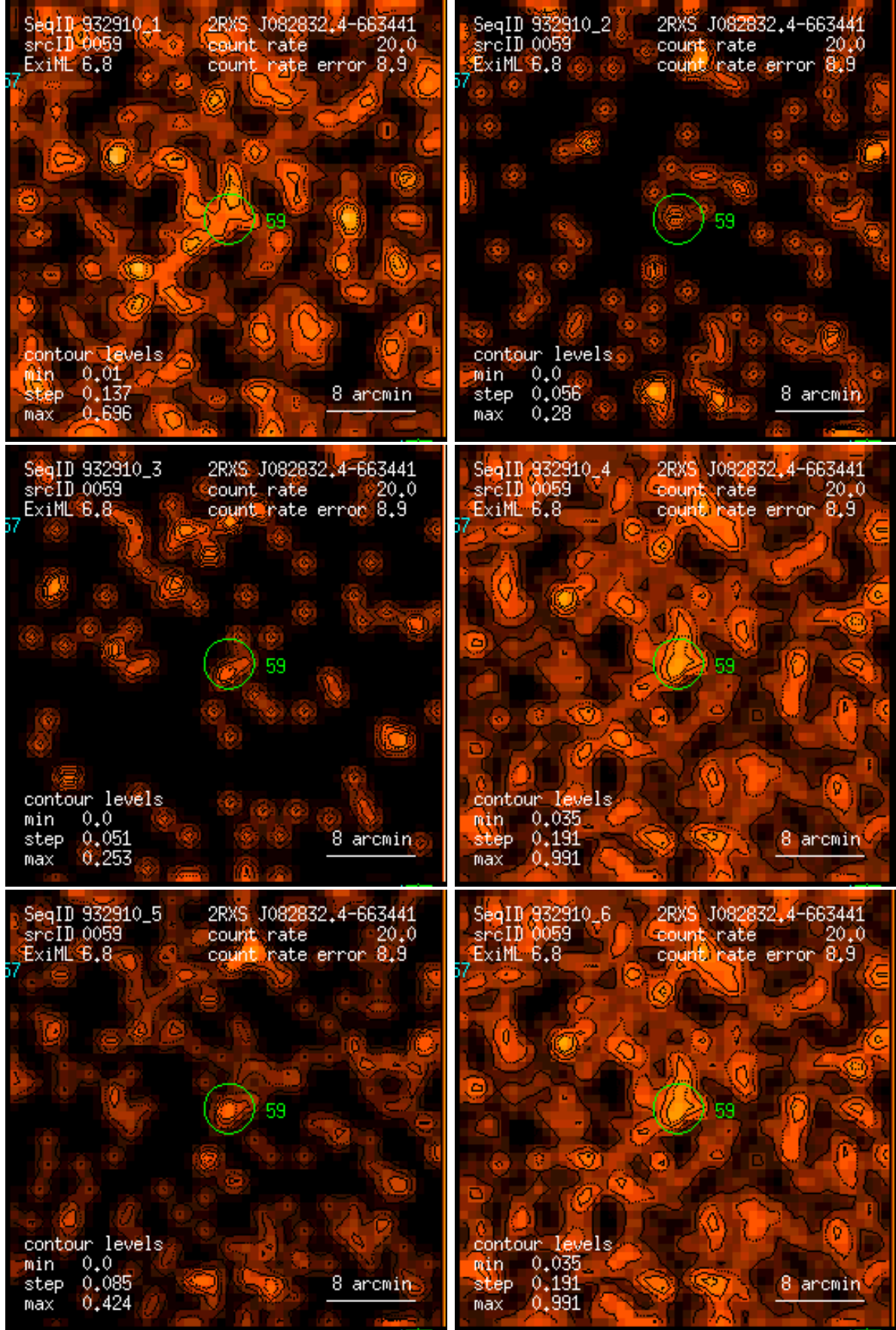
Figure 59: RASS 932910: detection 0059: band rate images, Gaussian filter: (1) PSPC channels 11 – 41, (2) 52 – 90, (3) 91 – 201, (4) 11 – 235, (5) 52 – 201, (6) 11 – 201. Broad band rates in counts/ks. Band rate contour levels in counts/ks/arcmin 2 .
