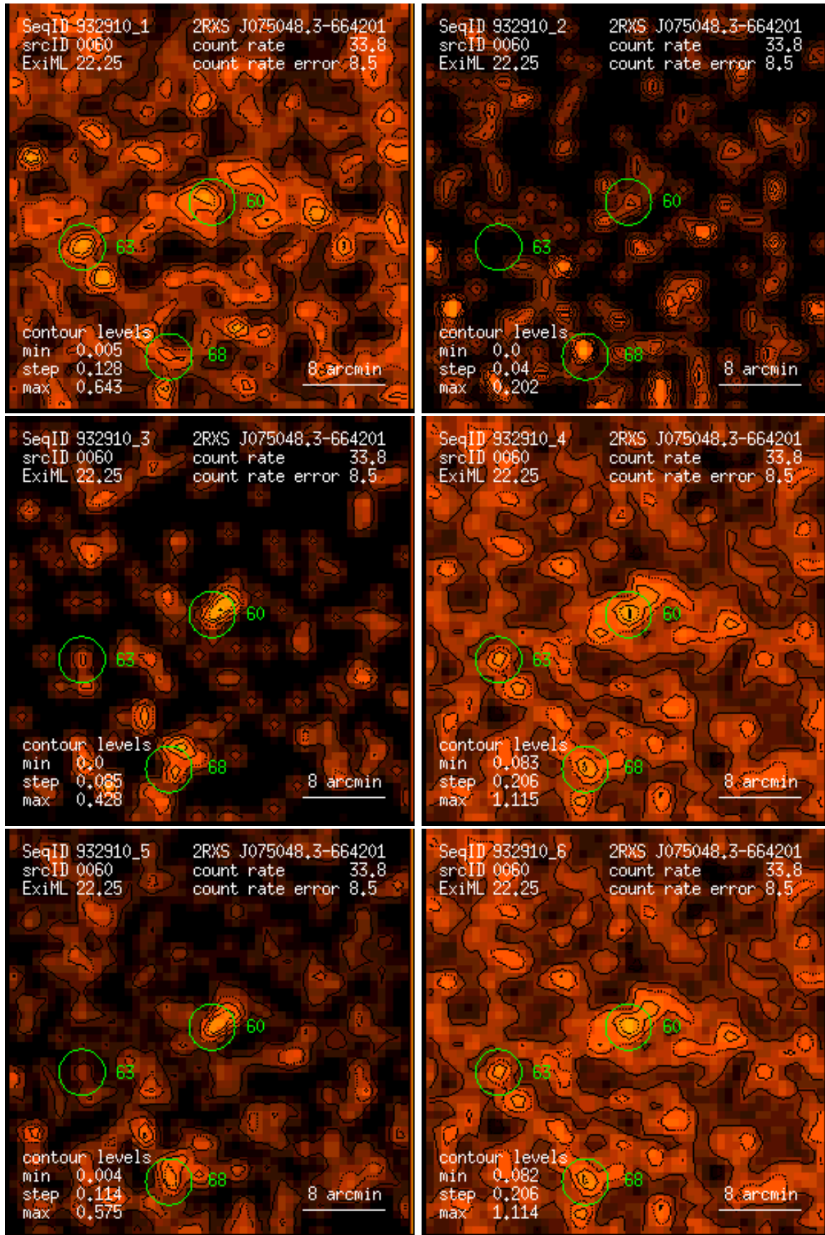
Figure 60: RASS 932910: detection 0060: band rate images, Gaussian filter: (1) PSPC channels 11 – 41, (2) 52 – 90, (3) 91 – 201, (4) 11 – 235, (5) 52 – 201, (6) 11 – 201. Broad band rates in counts/ks. Band rate contour levels in counts/ks/arcmin 2 .
