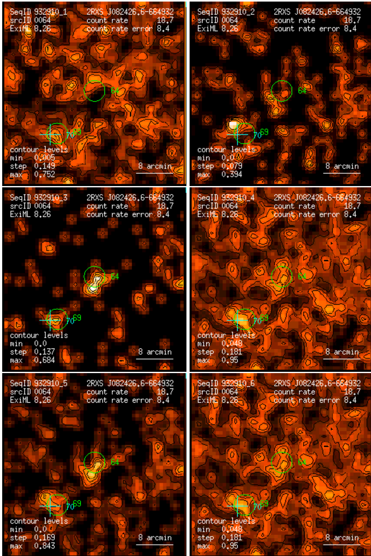
Figure 64: RASS 932910: detection 0064: band rate images, Gaussian filter: (1) PSPC channels 11 – 41, (2) 52 – 90, (3) 91 – 201, (4) 11 – 235, (5) 52 – 201, (6) 11 – 201. Broad band rates in counts/ks. Band rate contour levels in counts/ks/arcmin 2 .
