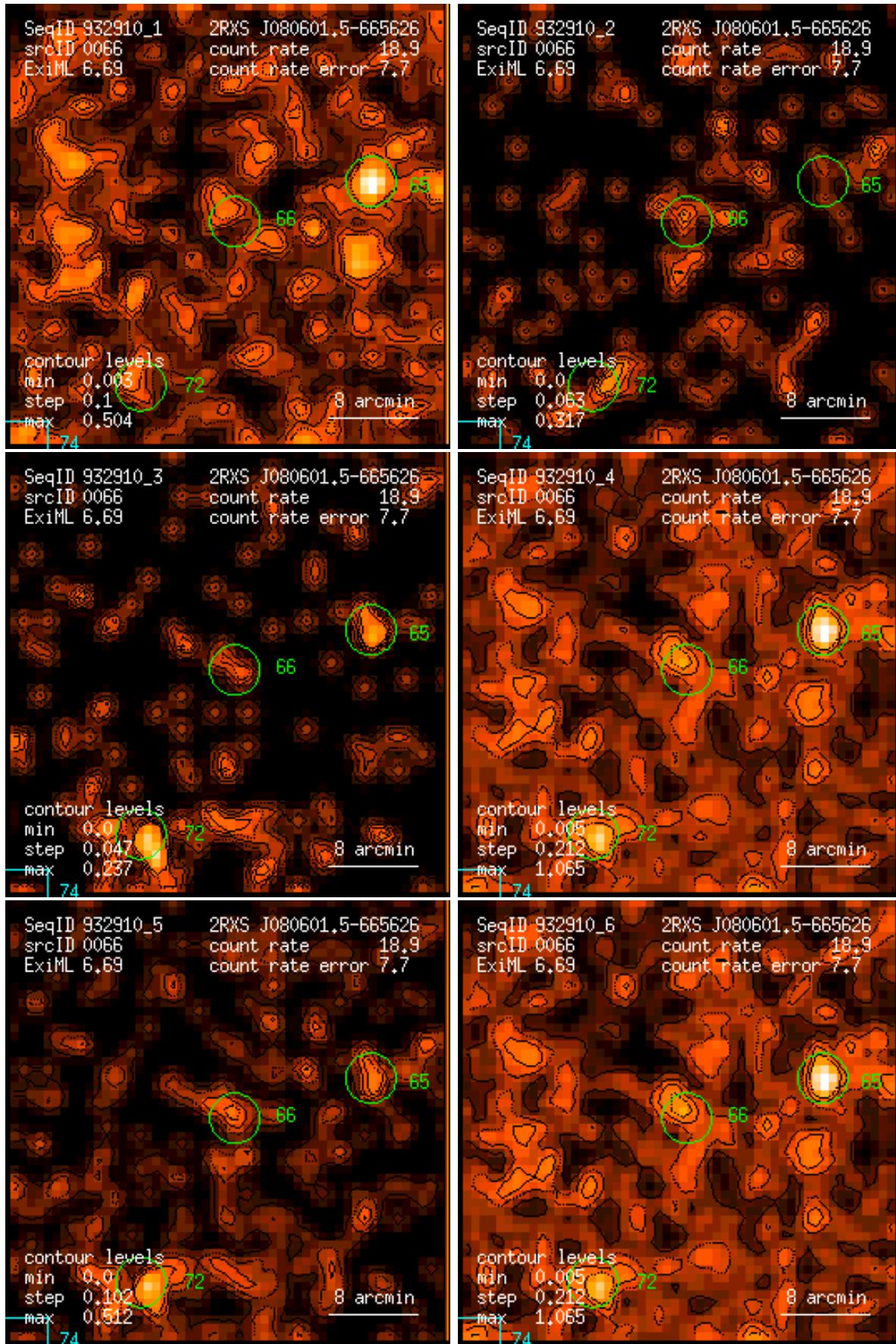
Figure 66: RASS 932910: detection 0066: band rate images, Gaussian filter: (1) PSPC channels 11 – 41, (2) 52 – 90, (3) 91 – 201, (4) 11 – 235, (5) 52 – 201, (6) 11 – 201. Broad band rates in counts/ks. Band rate contour levels in counts/ks/arcmin 2 .
